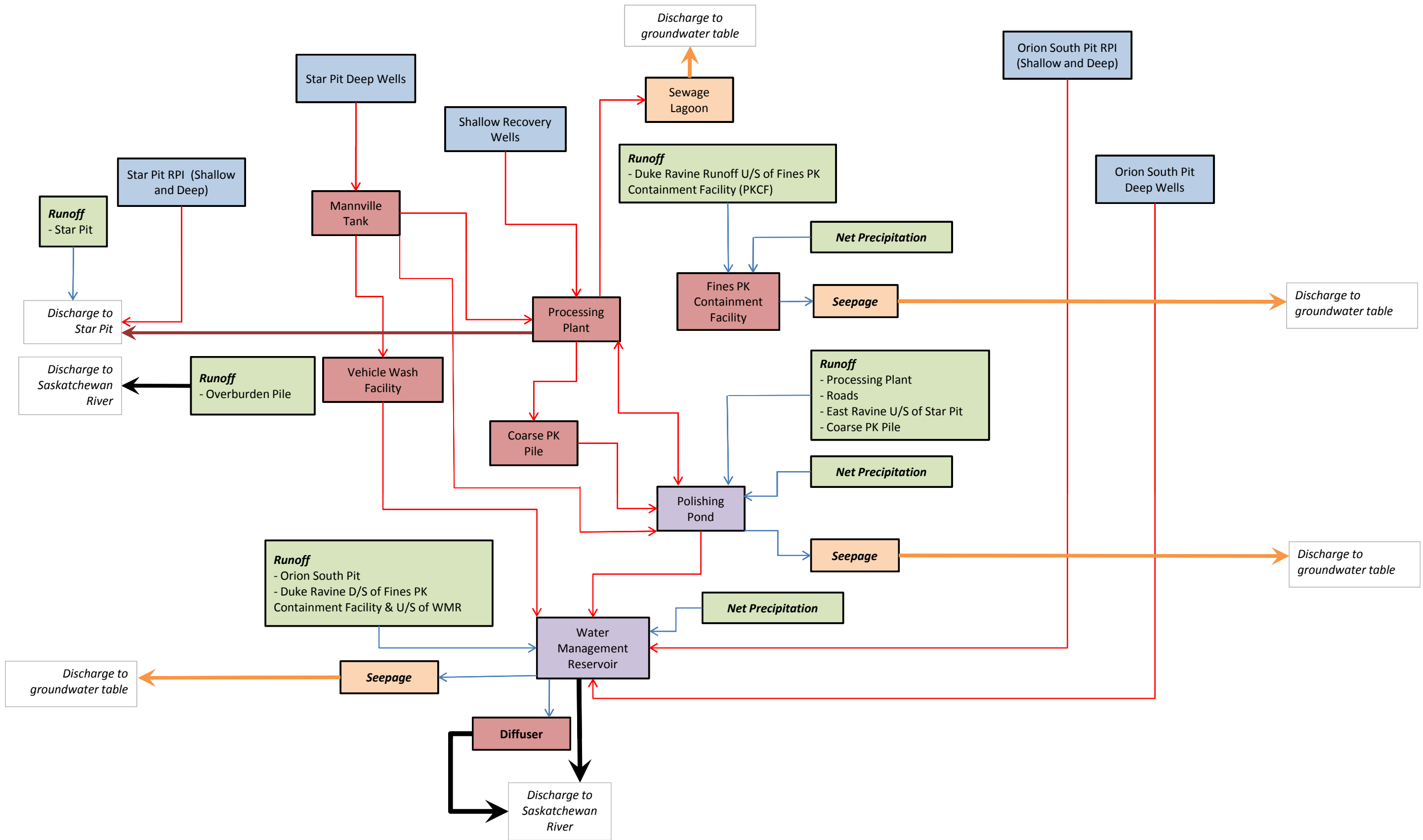
Figure 6.2.7-1: Shore Gold Water Quality Model Schematic Operation Phase (2015 - Summer 2035)
