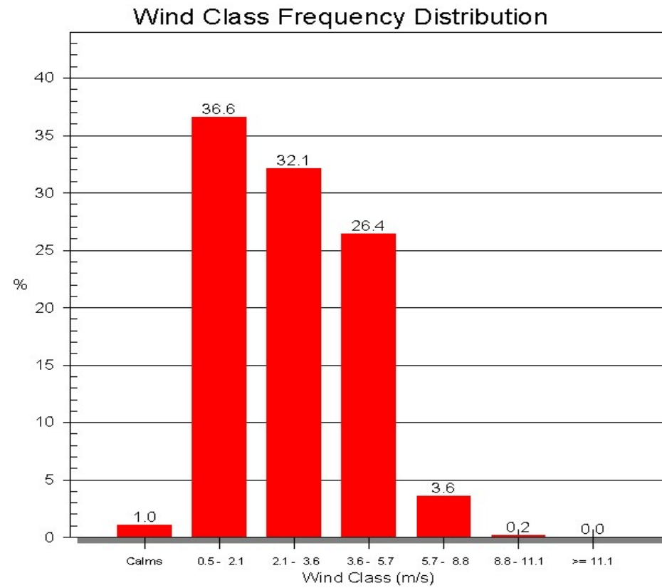
Figure 5.2.4-7: Wind Class Frequency Distribution for Fort à la Corne
