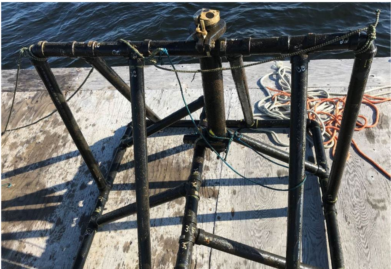
Figure 5: Nortek Aquadopp Acoustic Doppler Current Profiler and Mounting Frame Deployed at Patterson Lake North Intake
