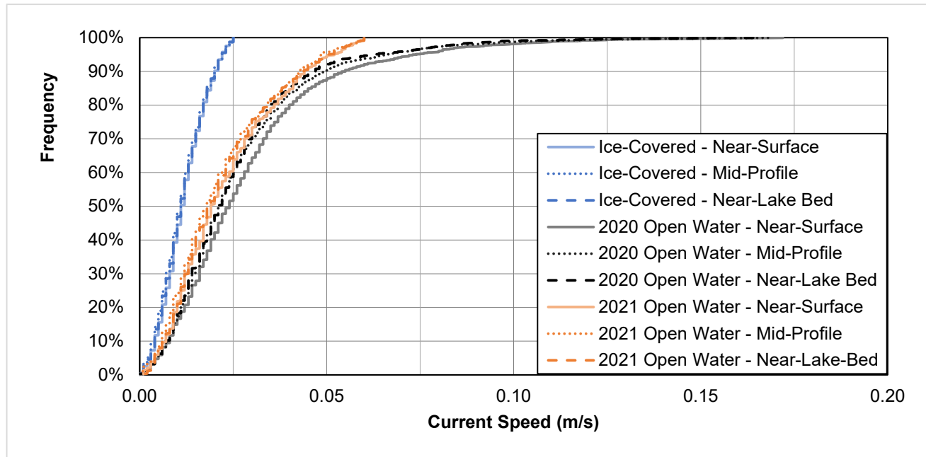
Figure 23: Cumulative Frequency Curve for Patterson Lake South
