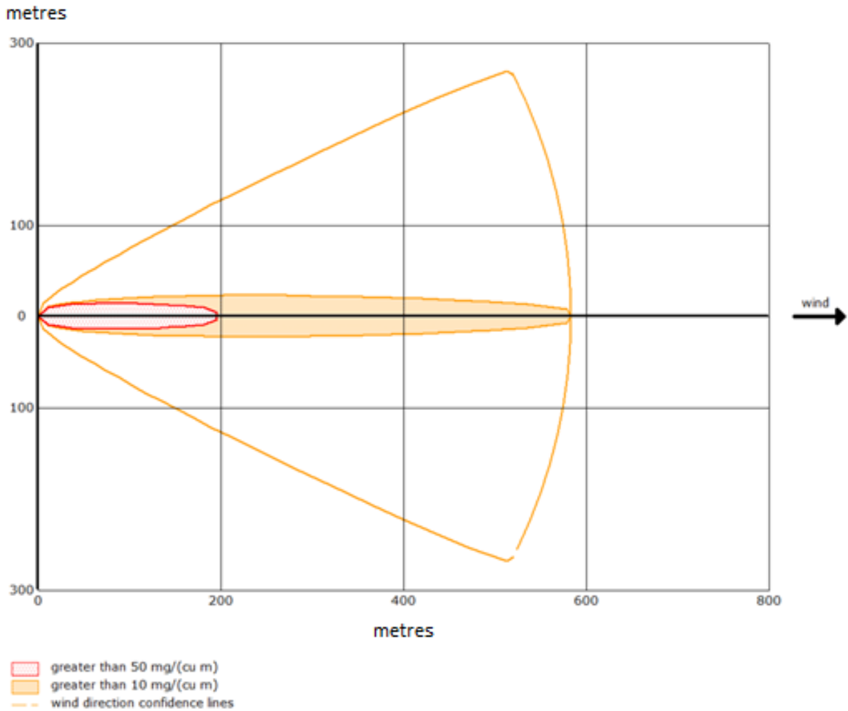
Figure 8-3: Concentration of Uranium in Air for Unconfined Fire for Worst-Case Weather Conditions
