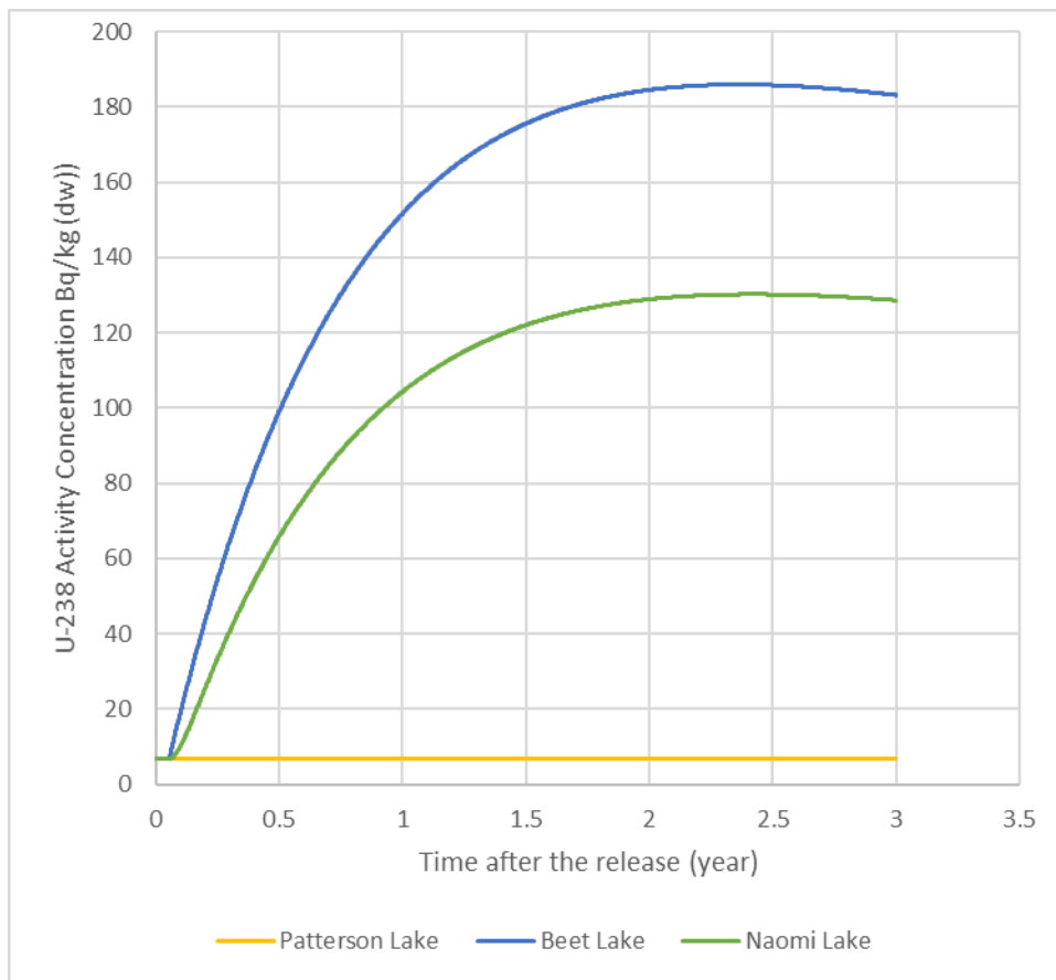
Figure 6-3: Long-Term Sediment Activity Concentrations of Uranium Following an Aquatic Release of Uranium Concentrate
