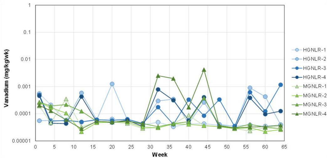
Figure F2-27: HCT Vanadium Mass Loading vs Time
