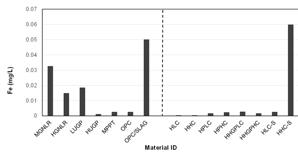
Figure D2-27: SFE Iron Concentration vs Material Type
