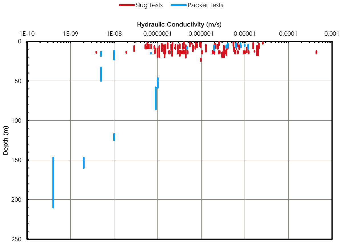
Figure 3.1 Hydraulic Conductivity Estimates in Bedrock
