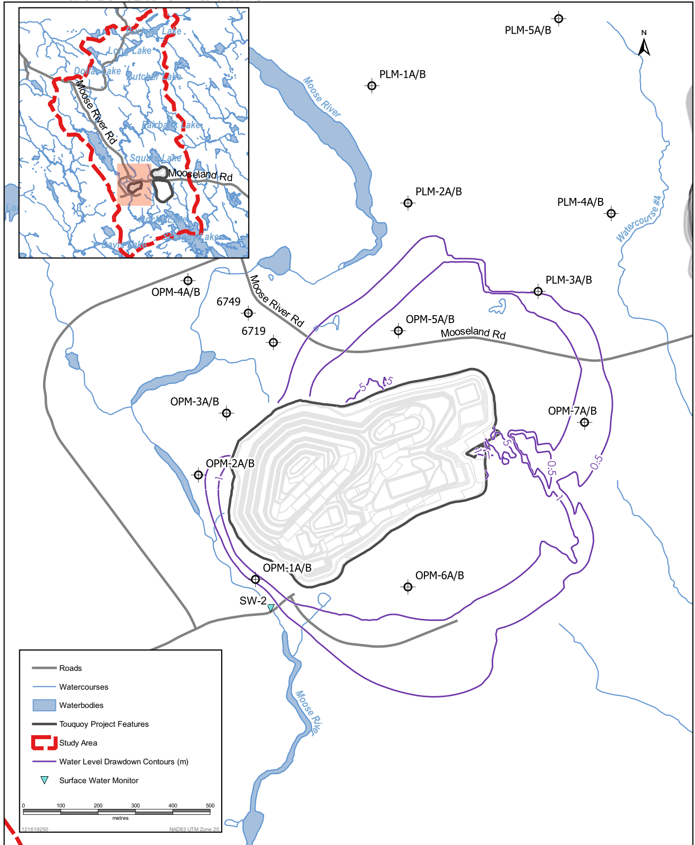
Drawdown at End of FMS Operations (Pit Lake Full)
