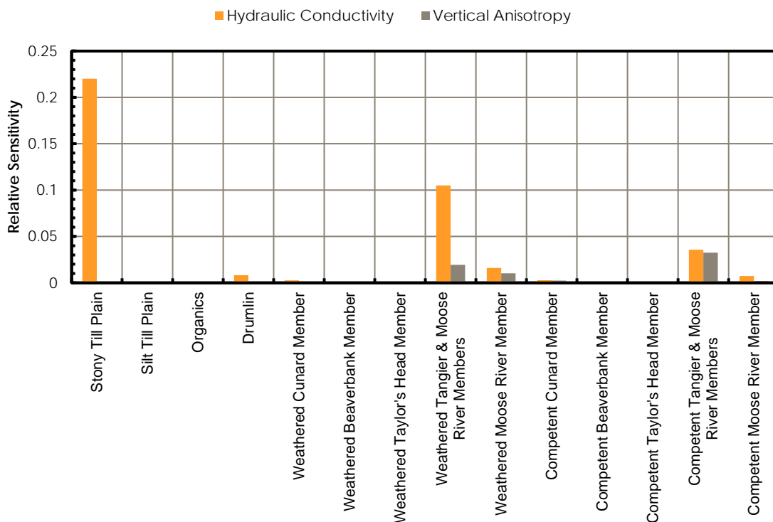
Figure 4.6 Calibration Sensitivity to Parameter Estimates
