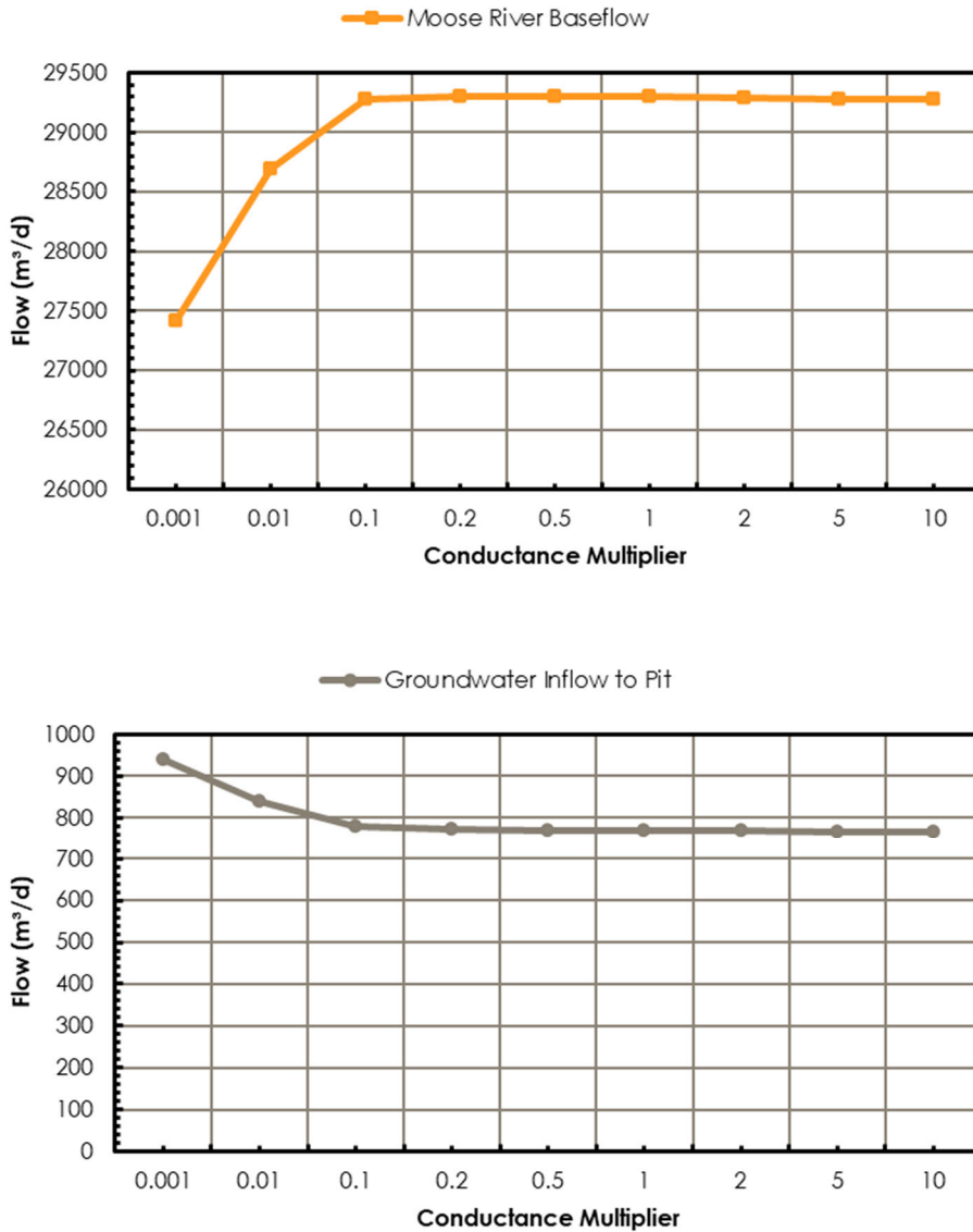
Figure 4.7 Sensitivity of Conductance to Calibrated Groundwater Flow Rates
