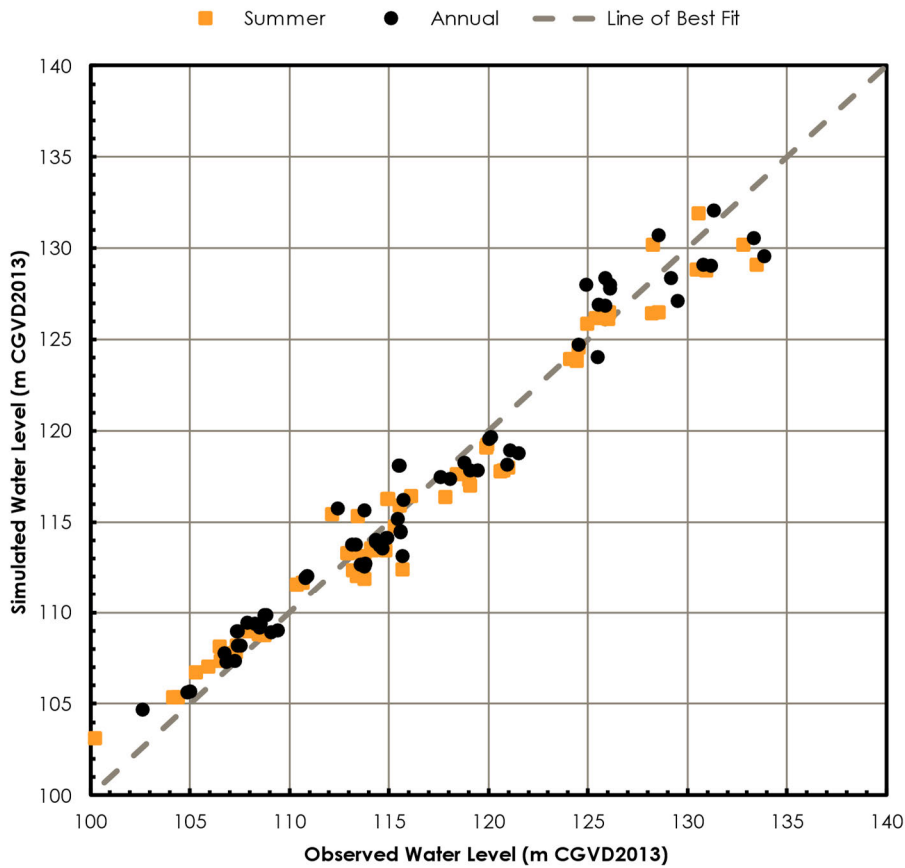
Figure 4.5 Scatterplot Showing the Match of Observed and Simulated Water Levels for Average Annual and Average Summer 2019 Conditions
