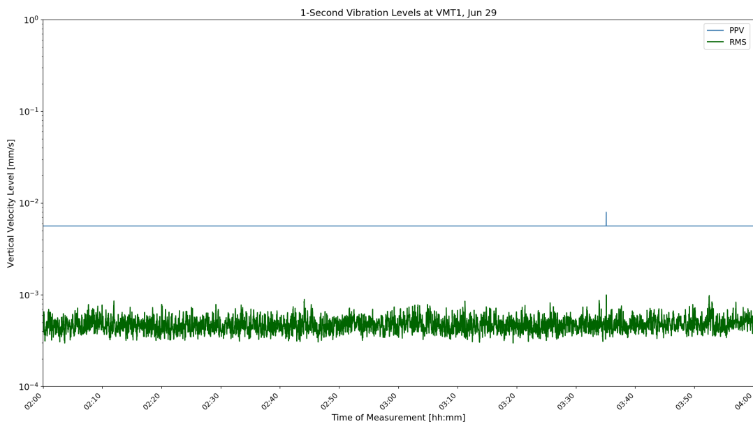
Figure D-27: VMT1 1-Second Velocity History Jun 29 22:00
