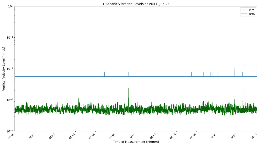
Figure D-4: VMT1 1-Second Velocity History Jun 23 04:00
