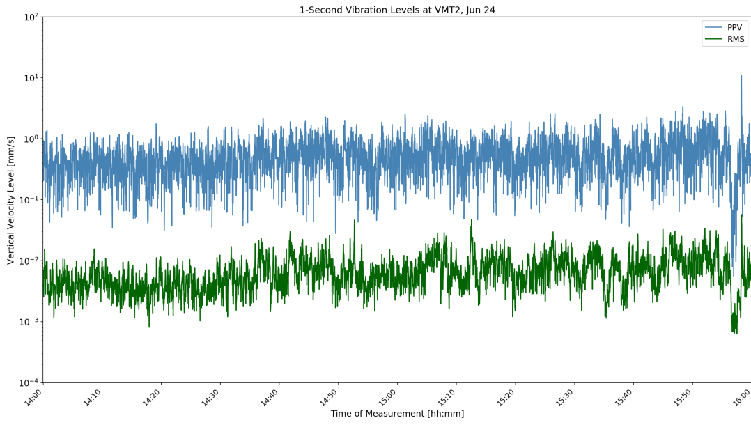
Figure D-37: VMT2 1-Second Velocity History Jun 24 10:00
