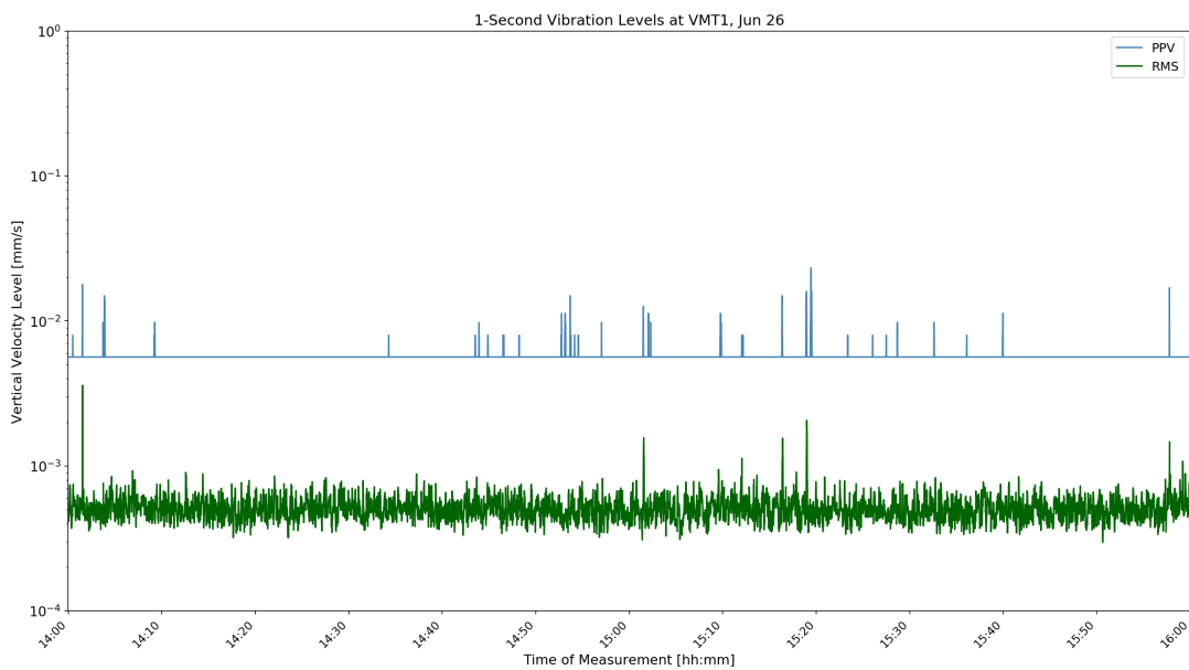
Figure D-17: VMT1 1-Second Velocity History Jun 26 10:00
