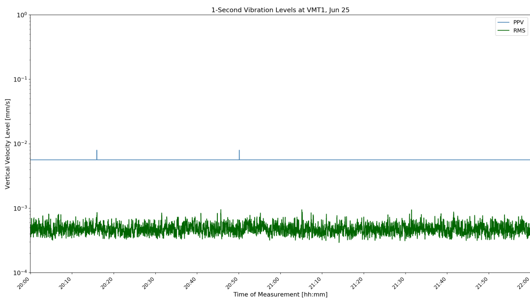
Figure D-14: VMT1 1-Second Velocity History Jun 25 16:00
