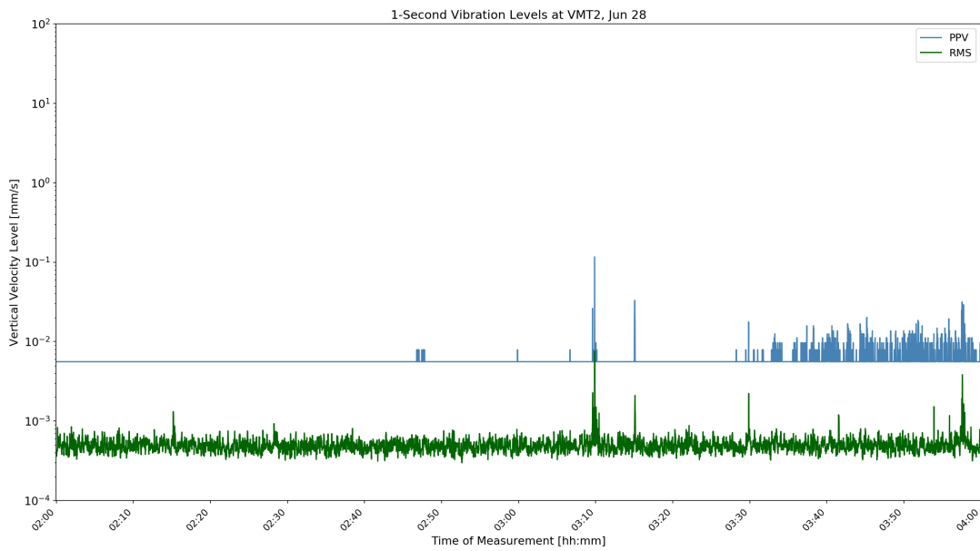
Figure D-51: VMT2 1-Second Velocity History Jun 28 22:00
