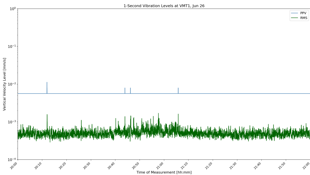
Figure D-18: VMT1 1-Second Velocity History Jun 26 16:00
