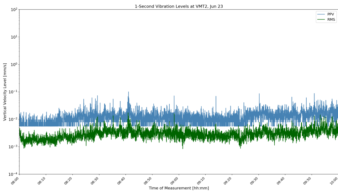
Figure D-32: VMT2 1-Second Velocity History Jun 23 04:00
