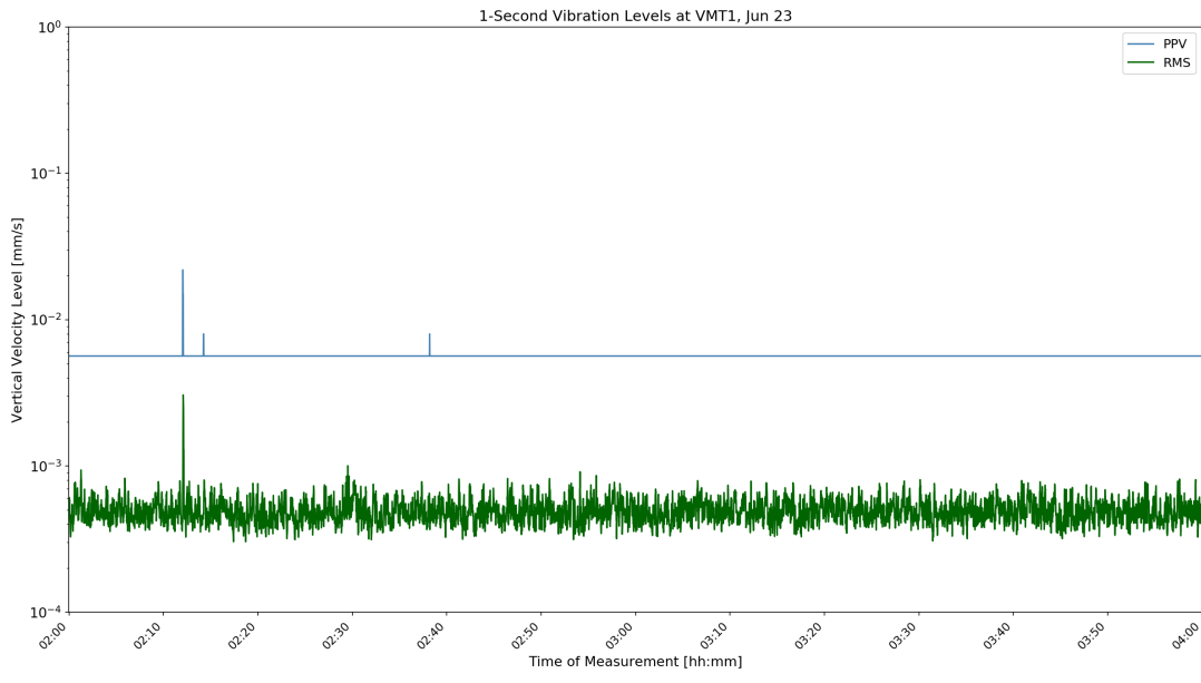
Figure D-3: VMT1 1-Second Velocity History Jun 23 22:00
