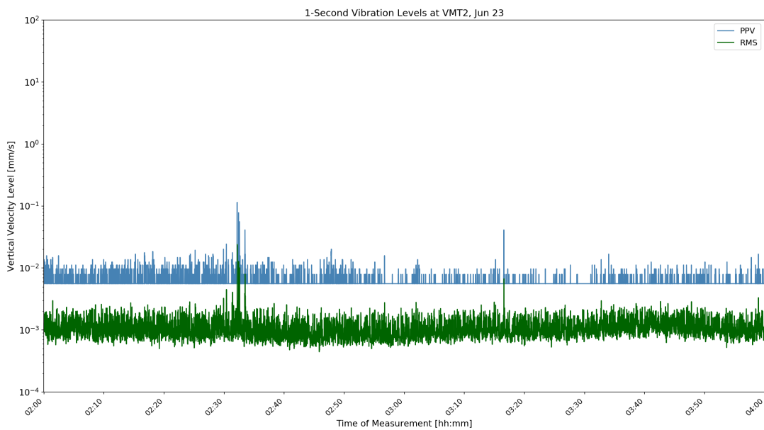
Figure D-31: VMT2 1-Second Velocity History Jun 23 22:00
