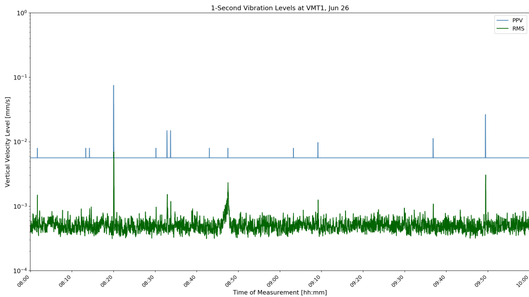
Figure D-16: VMT1 1-Second Velocity History Jun 26 04:00
