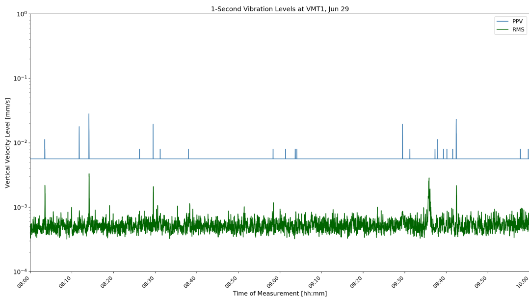
Figure D-28: VMT1 1-Second Velocity History Jun 29 04:00
