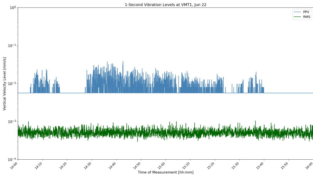
Figure D-1: VMT1 1-Second Velocity History Jun 22 10:00
