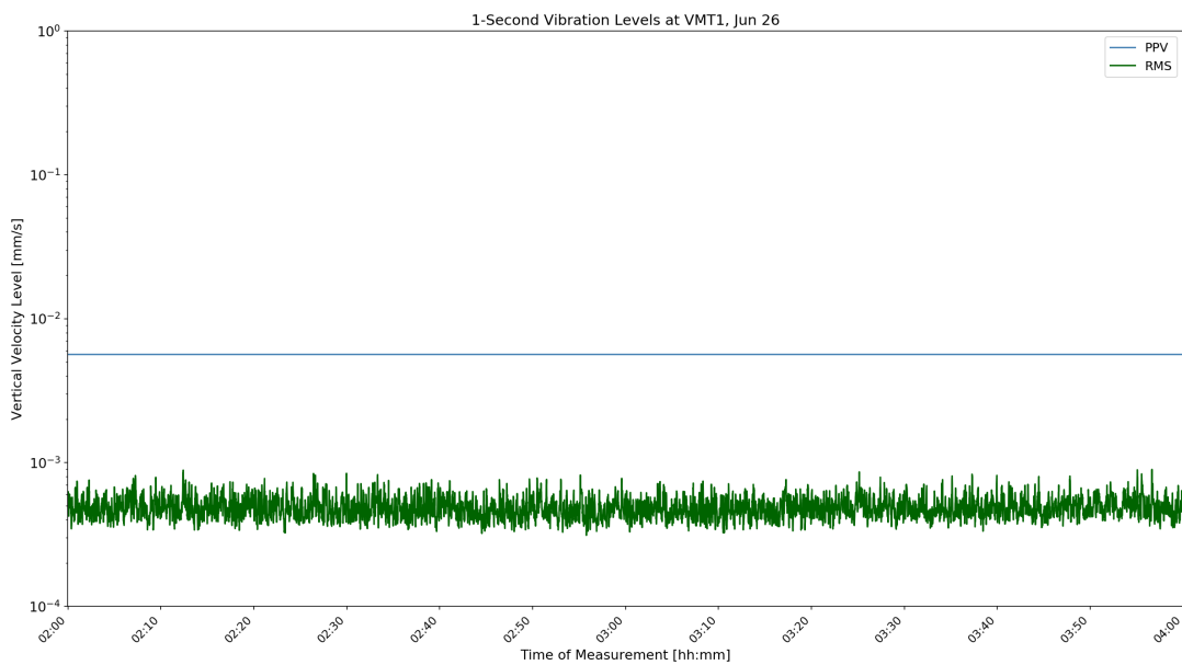
Figure D-15: VMT1 1-Second Velocity History Jun 26 22:00
