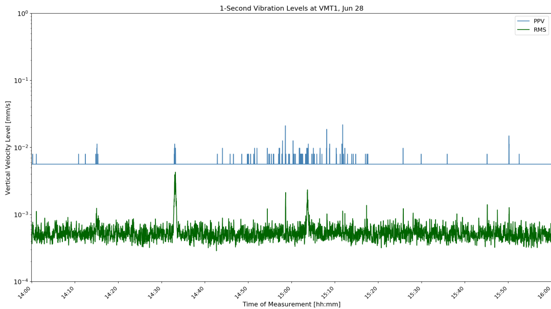
Figure D-25: VMT1 1-Second Velocity History Jun 28 10:00
