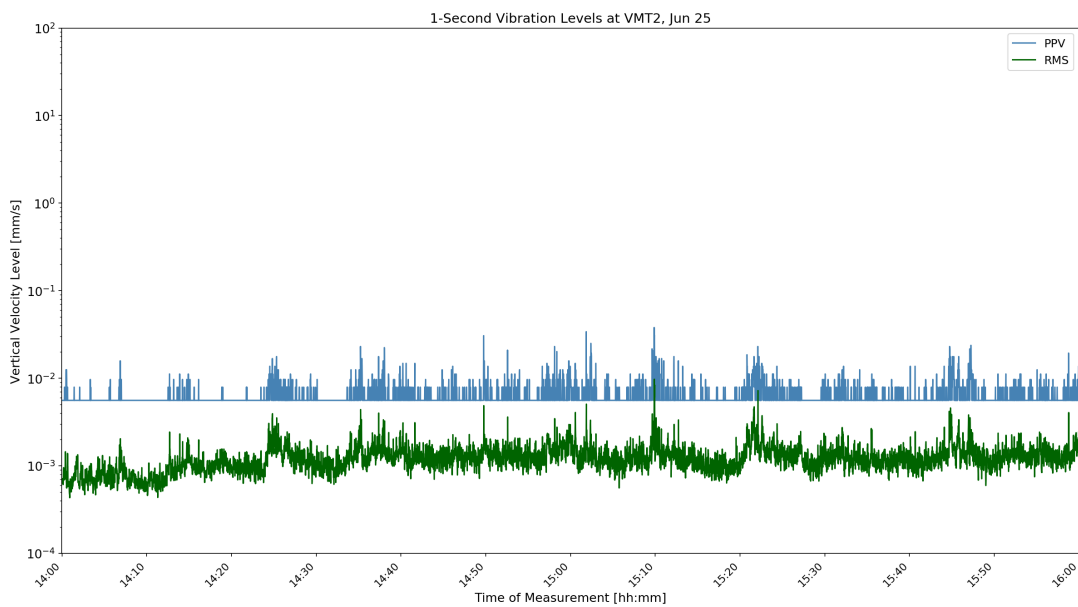
Figure D-41: VMT2 1-Second Velocity History Jun 25 10:00
