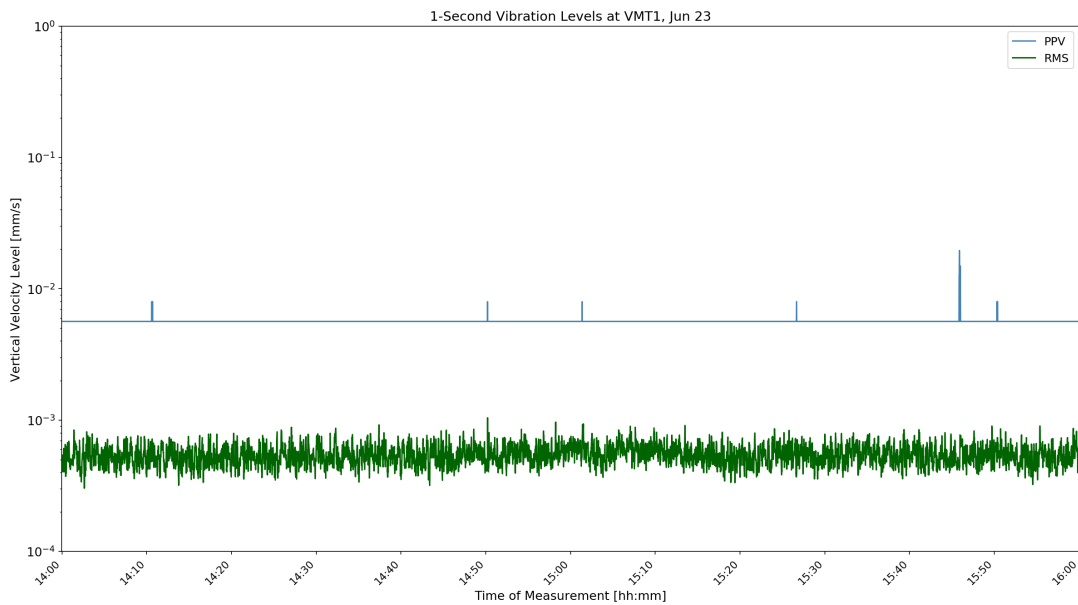
Figure D-5: VMT1 1-Second Velocity History Jun 23 10:00
