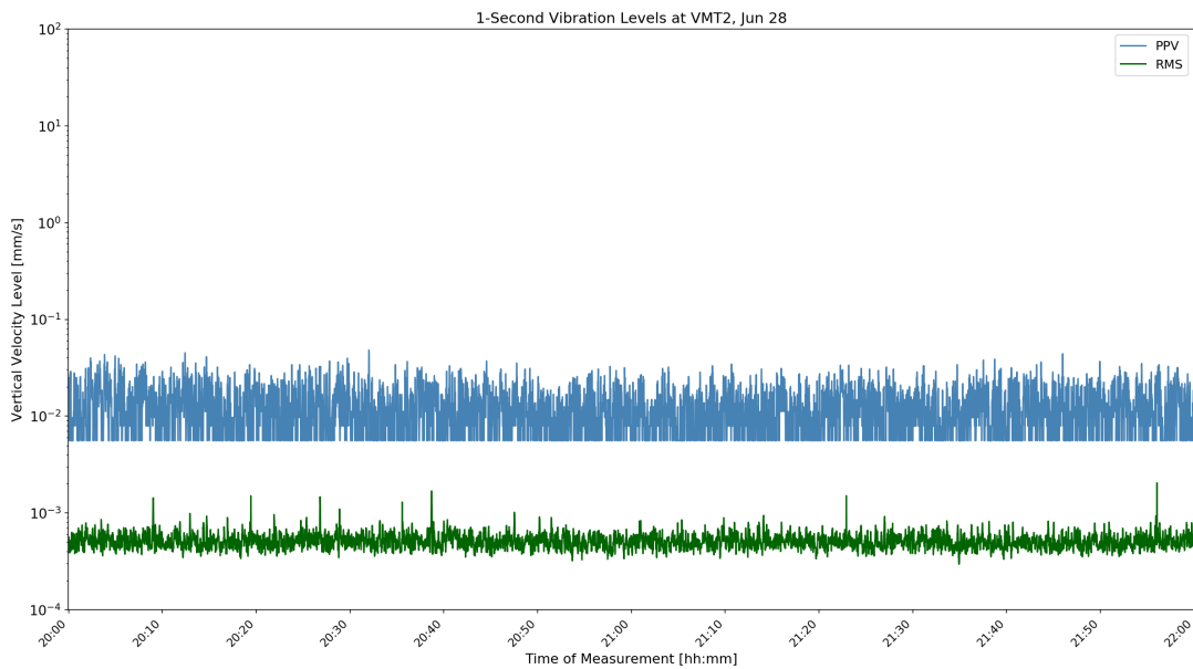
Figure D-54: VMT2 1-Second Velocity History Jun 28 16:00
