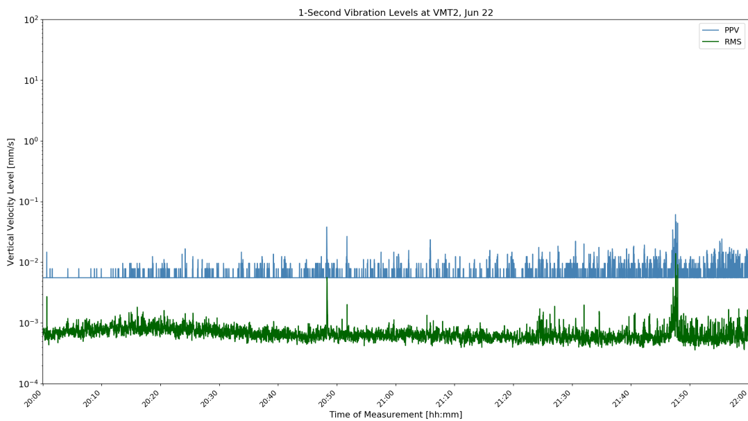
Figure D-30: VMT2 1-Second Velocity History Jun 22 16:00
