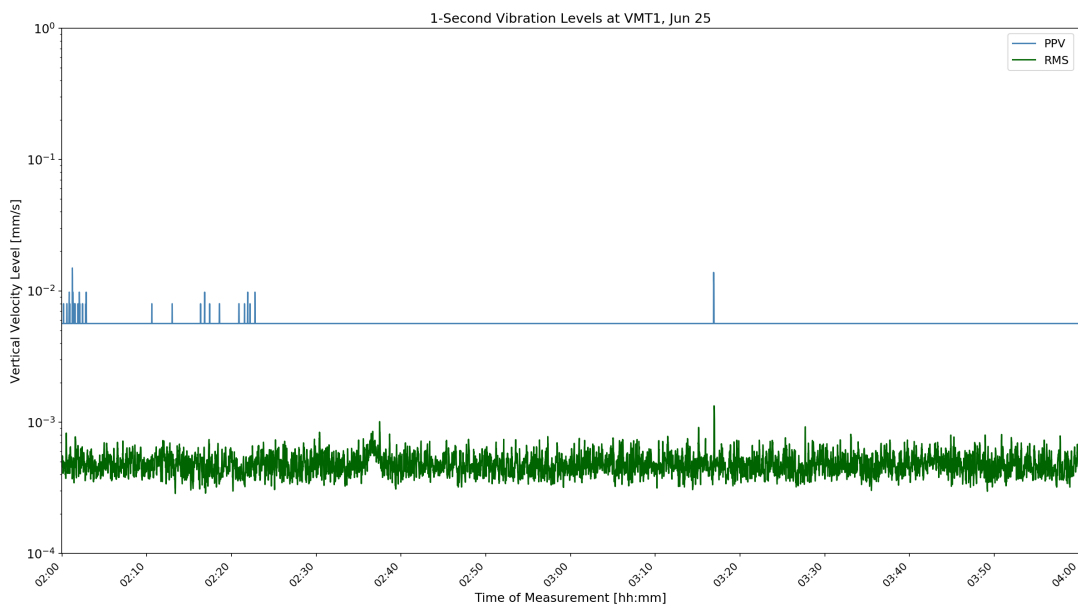
Figure D-11: VMT1 1-Second Velocity History Jun 25 22:00
