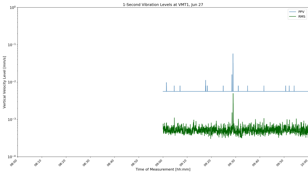
Figure D-20: VMT1 1-Second Velocity History Jun 27 04:00
