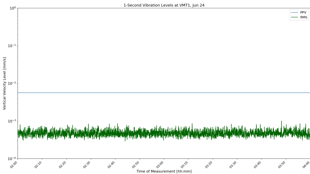
Figure D-7: VMT1 1-Second Velocity History Jun 24 22:00
