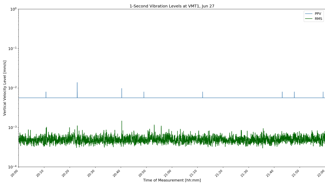
Figure D-22: VMT1 1-Second Velocity History Jun 27 16:00
