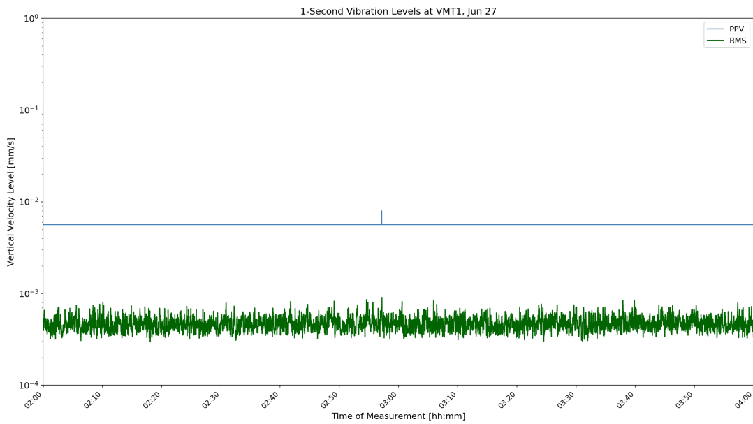
Figure D-19: VMT1 1-Second Velocity History Jun 27 22:00
