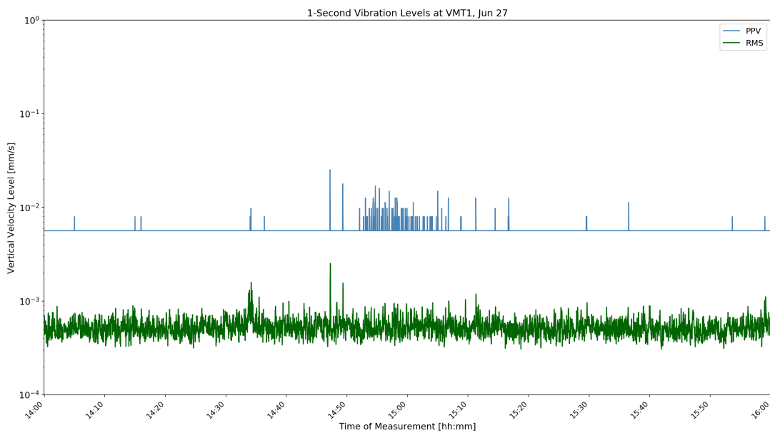
Figure D-21: VMT1 1-Second Velocity History Jun 27 10:00
