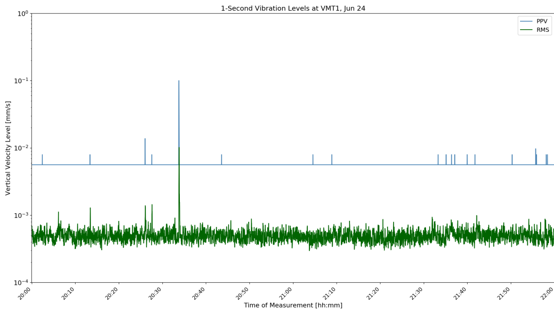
Figure D-10: VMT1 1-Second Velocity History Jun 24 16:00
