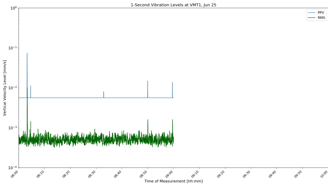
Figure D-12: VMT1 1-Second Velocity History Jun 25 04:00
