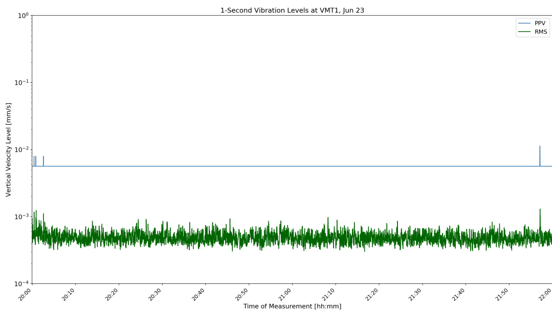
Figure D-6: VMT1 1-Second Velocity History Jun 23 16:00
