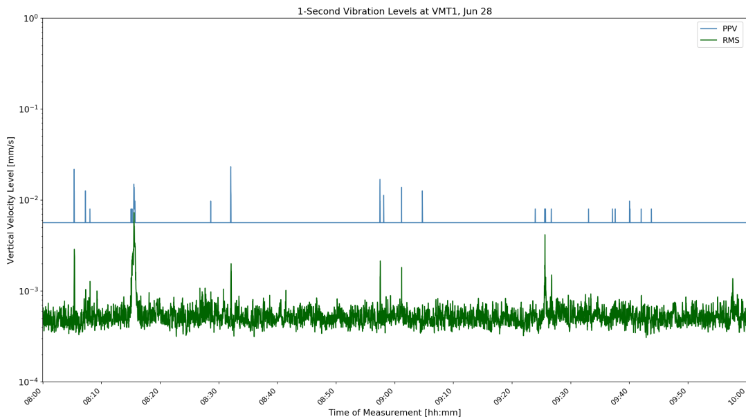
Figure D-24: VMT1 1-Second Velocity History Jun 28 04:00
