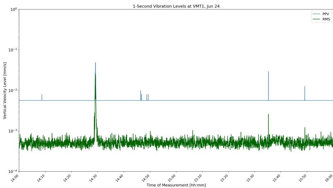
Figure D-9: VMT1 1-Second Velocity History Jun 24 10:00
