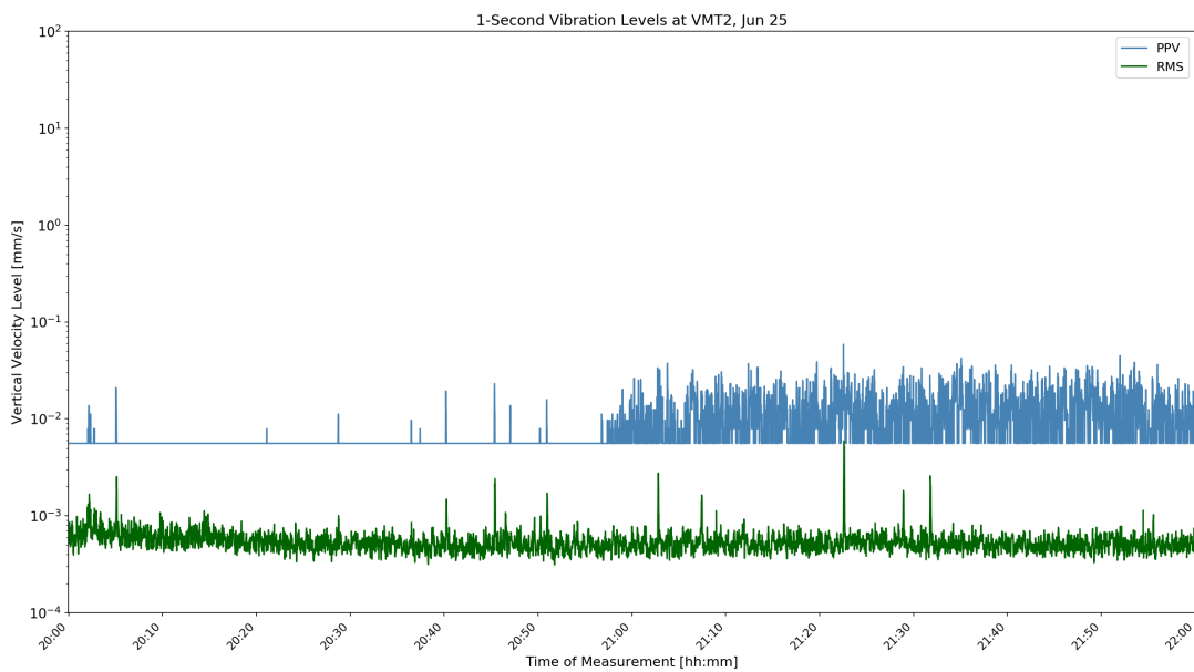
Figure D-42: VMT2 1-Second Velocity History Jun 25 16:00
