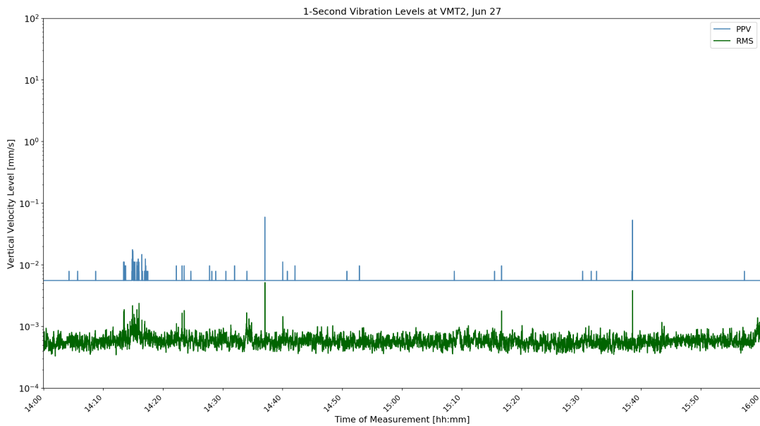
Figure D-49: VMT2 1-Second Velocity History Jun 27 10:00
