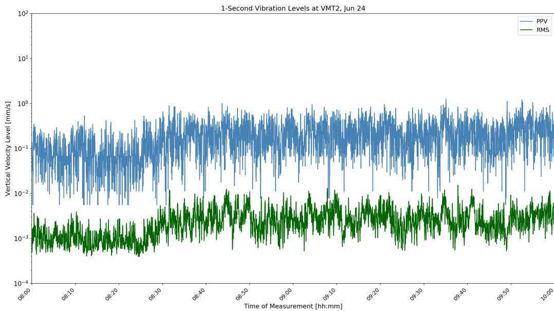
Figure D-36: VMT2 1-Second Velocity History Jun 24 04:00
