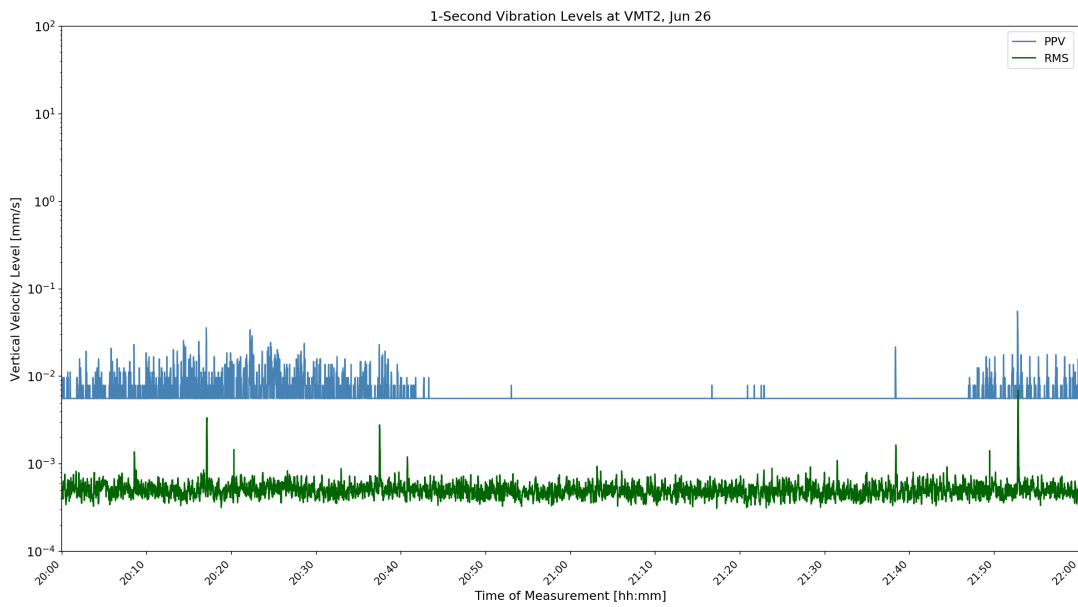
Figure D-46: VMT2 1-Second Velocity History Jun 26 16:00
