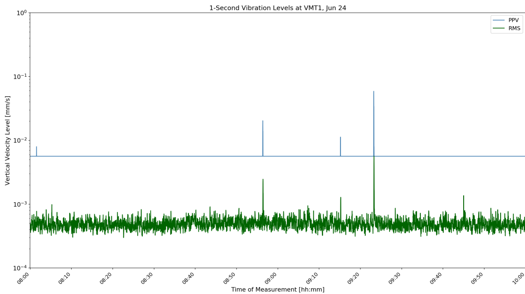
Figure D-8: VMT1 1-Second Velocity History Jun 24 04:00
