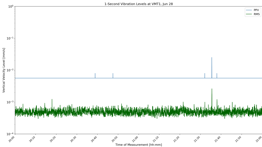
Figure D-26: VMT1 1-Second Velocity History Jun 28 16:00
