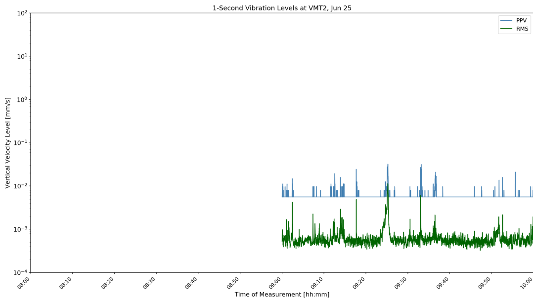
Figure D-40: VMT2 1-Second Velocity History Jun 25 04:00
