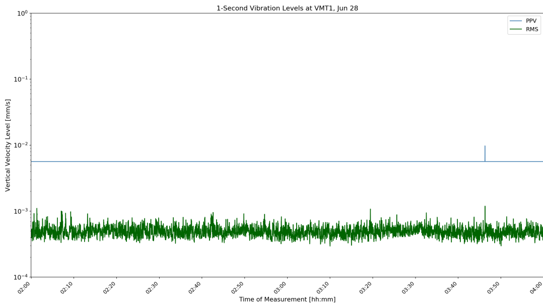
Figure D-23: VMT1 1-Second Velocity History Jun 28 22:00
