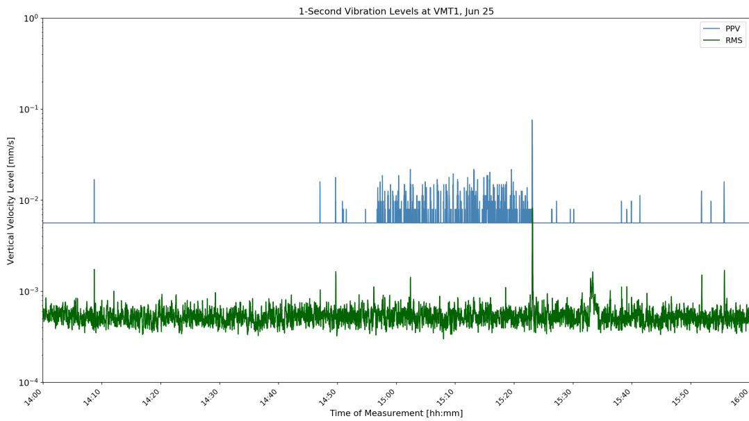
Figure D-13: VMT1 1-Second Velocity History Jun 25 10:00
