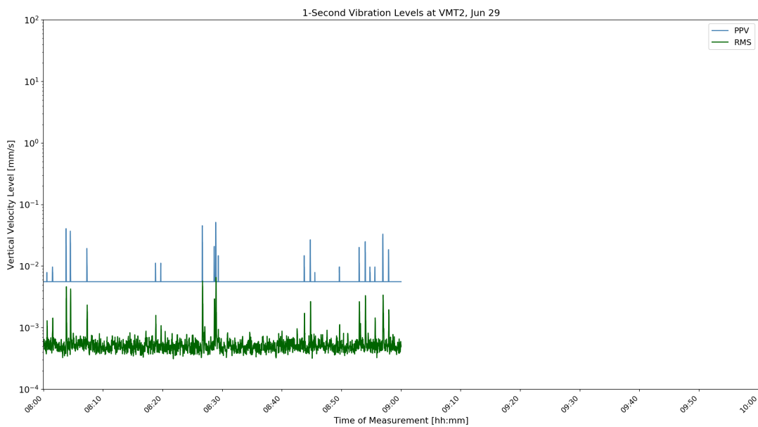
Figure D-56: VMT2 1-Second Velocity History Jun 29 04:00
