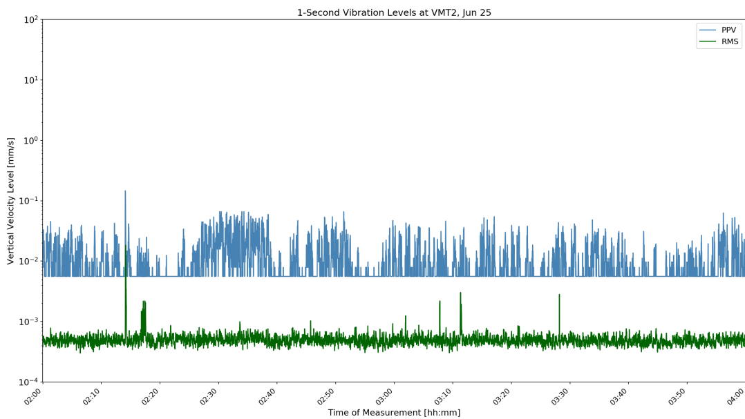
Figure D-39: VMT2 1-Second Velocity History Jun 25 22:00
