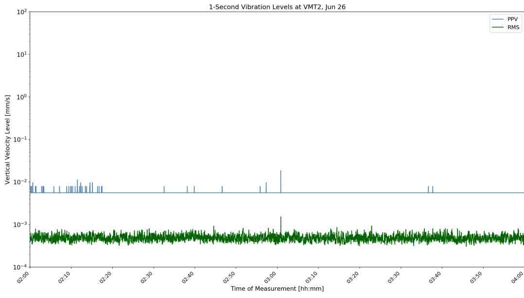
Figure D-43: VMT2 1-Second Velocity History Jun 26 22:00
