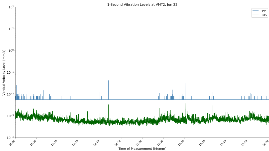
Figure D-29: VMT2 1-Second Velocity History Jun 22 10:00
