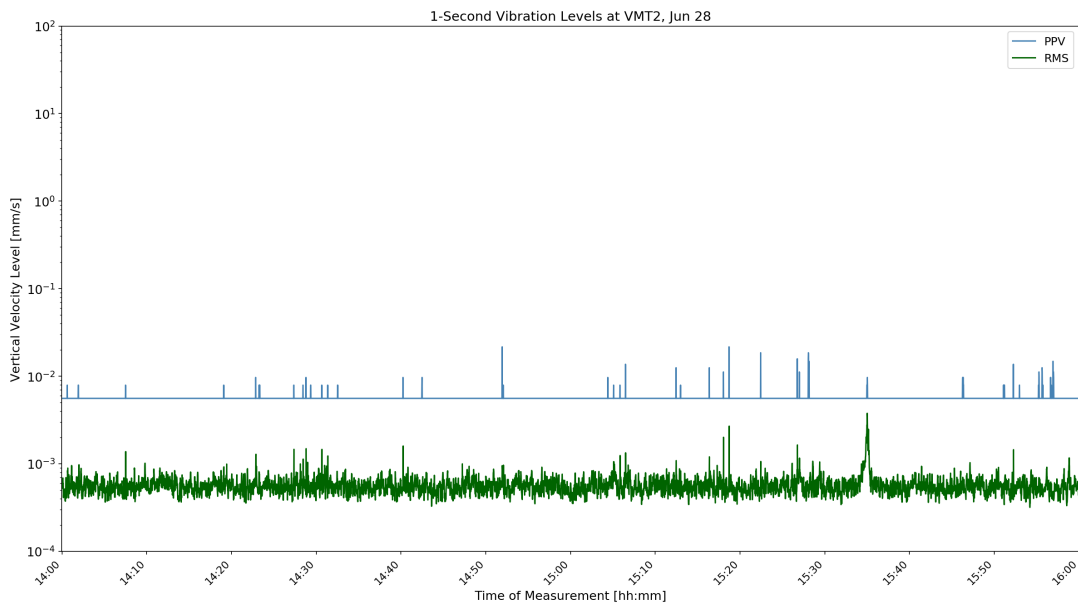
Figure D-53: VMT2 1-Second Velocity History Jun 28 10:00
