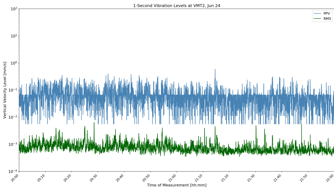
Figure D-38: VMT2 1-Second Velocity History Jun 24 16:00
