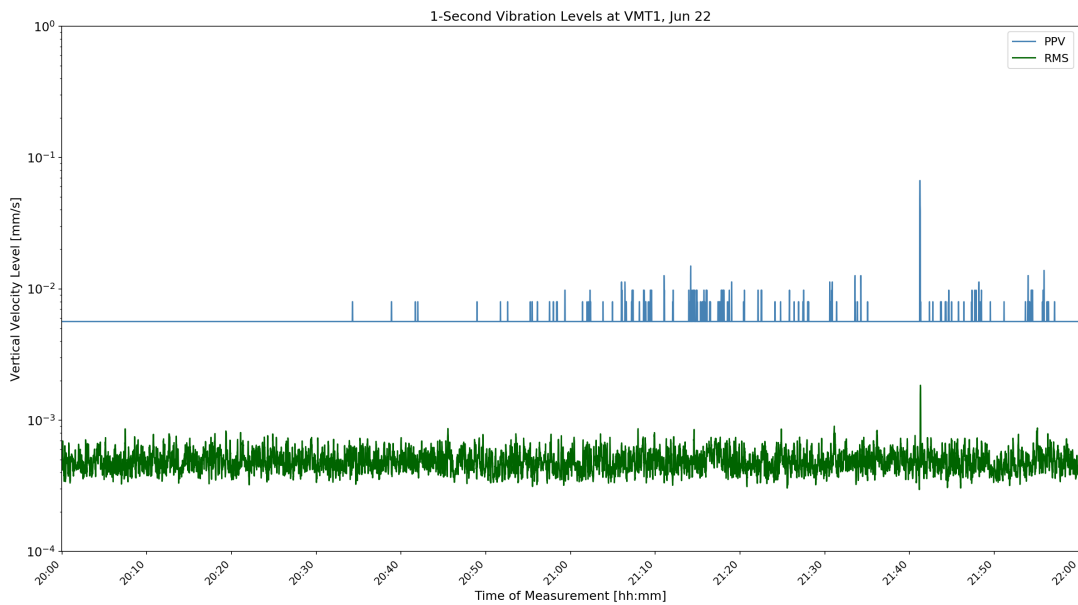
Figure D-2: VMT1 1-Second Velocity History Jun 22 16:00
