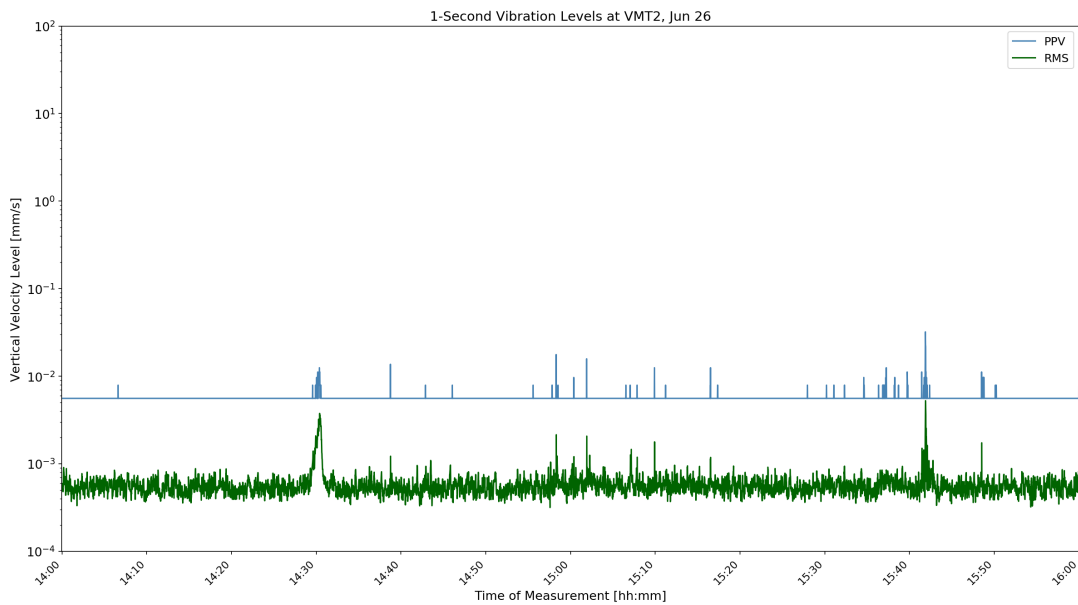
Figure D-45: VMT2 1-Second Velocity History Jun 26 10:00
