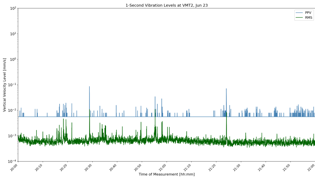
Figure D-34: VMT2 1-Second Velocity History Jun 23 16:00
