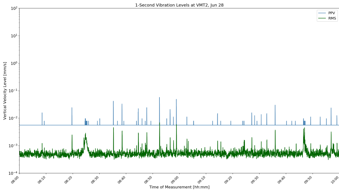
Figure D-52: VMT2 1-Second Velocity History Jun 28 04:00
