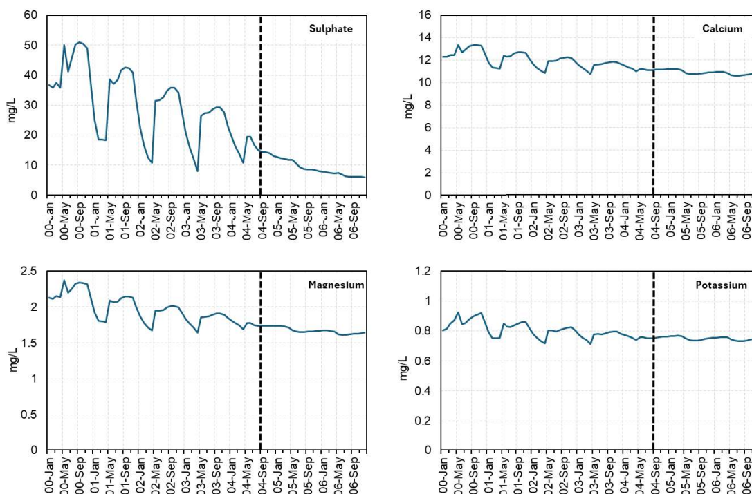
Figure 4-9: Predictions of sulphate, calcium, magnesium and potassium concentrations in the surface mixed layer (uppermost 20 to 40 m) of the open pit basin. Timing of basin connection to Springpole Lake shown as vertical black dashed line (4.8 years). All values expressed as totals in mg/L.
