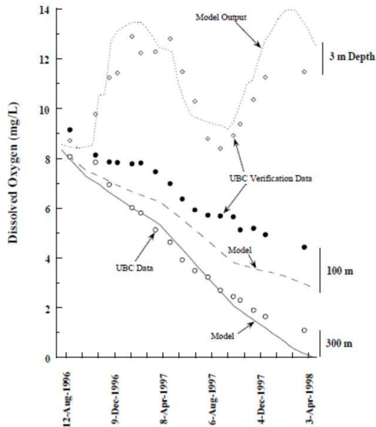
Figure 2-3: Modeled (PitMod) versus measured dissolved oxygen concentrations at three depths in the Island Copper Pit Lake, spanning a two-year period from 1996 to 1998 (plot from Crusius et al. , 2002a). UBC = University of British Columbia.
