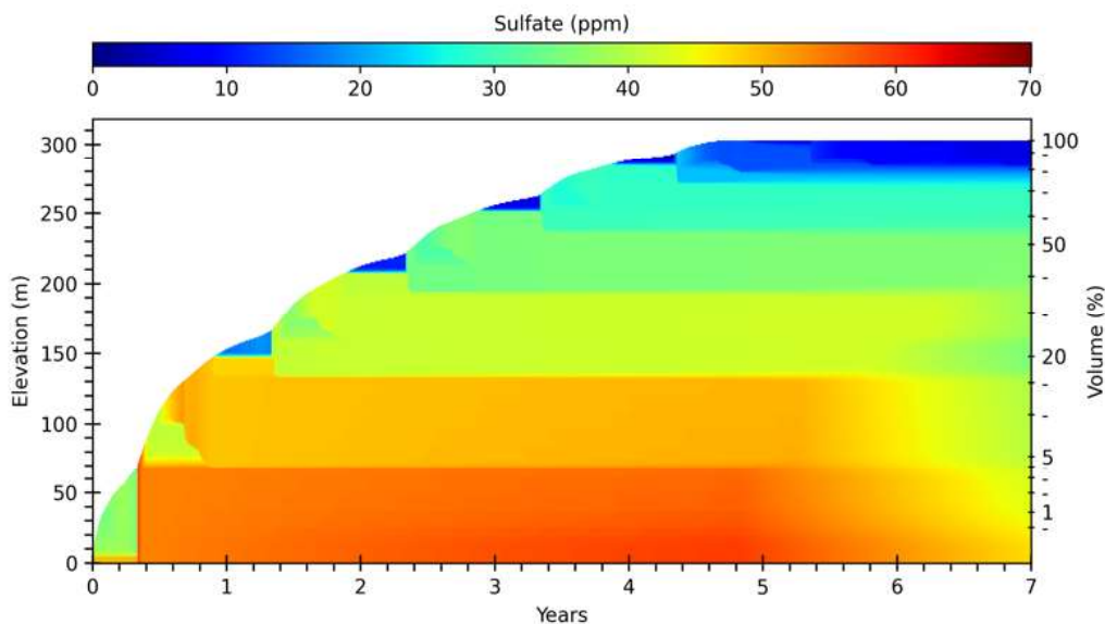
Figure 4-8: Predictions of the vertical and temporal evolution of sulfate for the open pit basin. Predictions are shown as a function of depth (primary Y-axis), pit volume % (secondary Y-axis) and time (X-axis). Values in ppm or mg/L.
