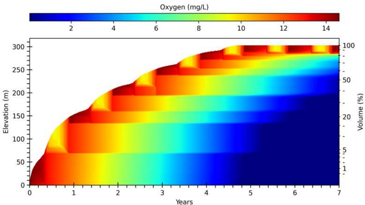
Figure 4-5: Predictions of the vertical and temporal evolution of dissolved oxygen for the open pit basin. Predictions are shown as a function of depth (primary Y-axis), pit volume % (secondary Y-axis) and time (X-axis).
