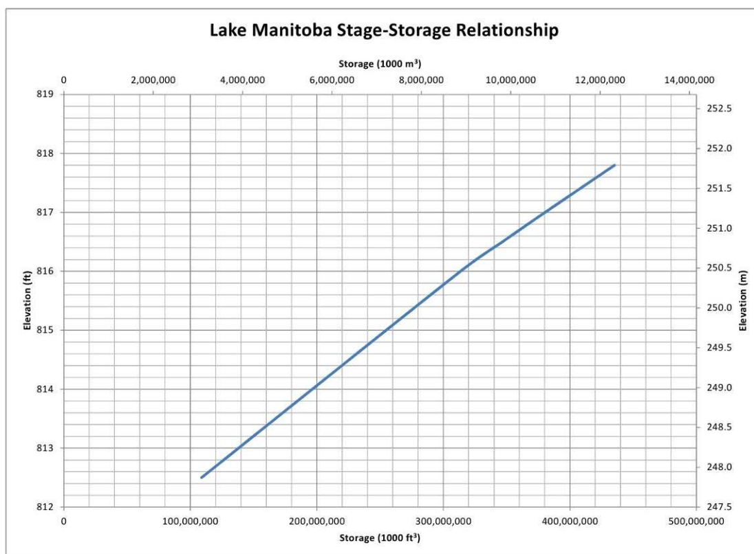
Figure 7 – Lake Manitoba Stage-Storage Relationship
