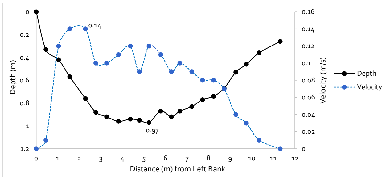
Appendix B-1. Cross-sectional profile of Transect 1 on Watchorn Creek.
