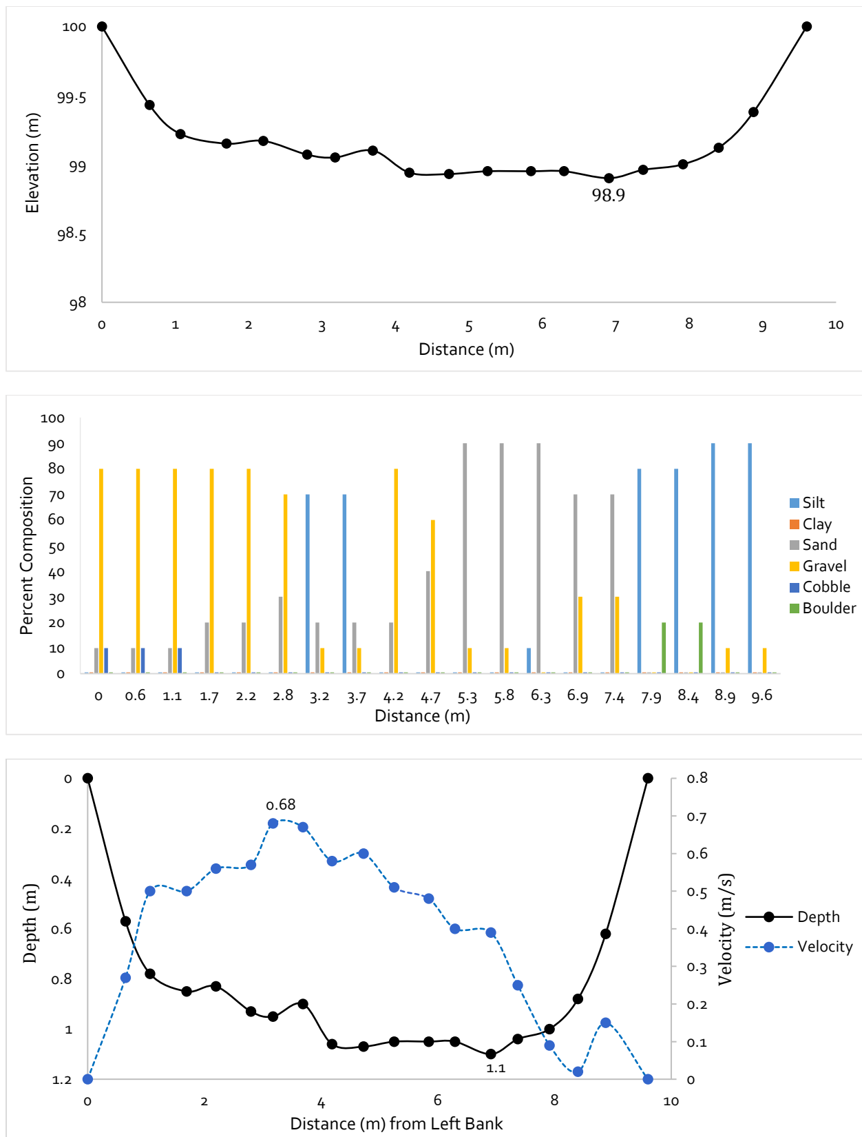
Appendix B-8. Cross-sectional profile, substrate, and velocity of Transect 1 on Birch Creek.
