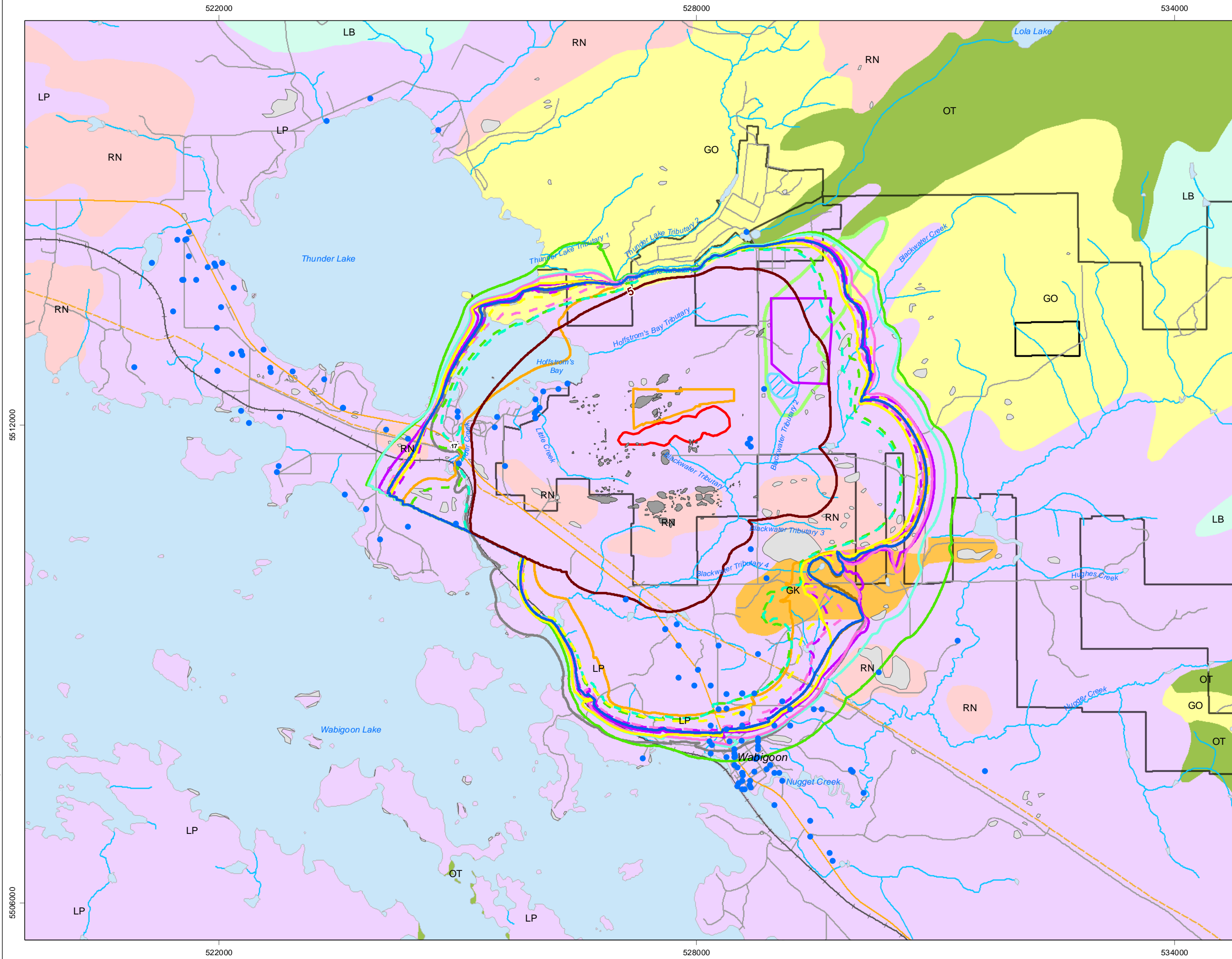
Figure 21 Model predicted ZOIs (1m drawdown) in Basal Sand/Shallow Bedrock Units
