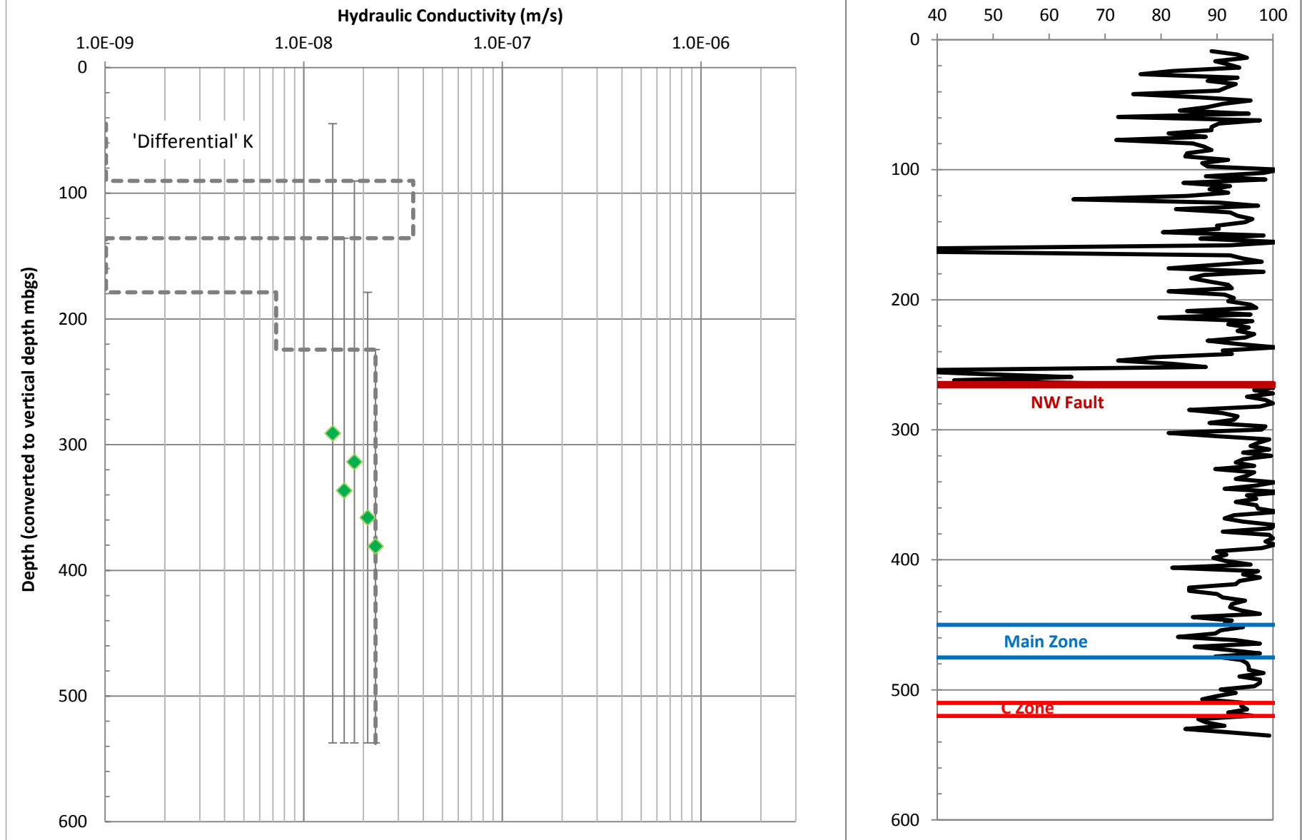
Figure 12c Packer Test Results for Existing Exploration Boreholes from West to East - TL11195
