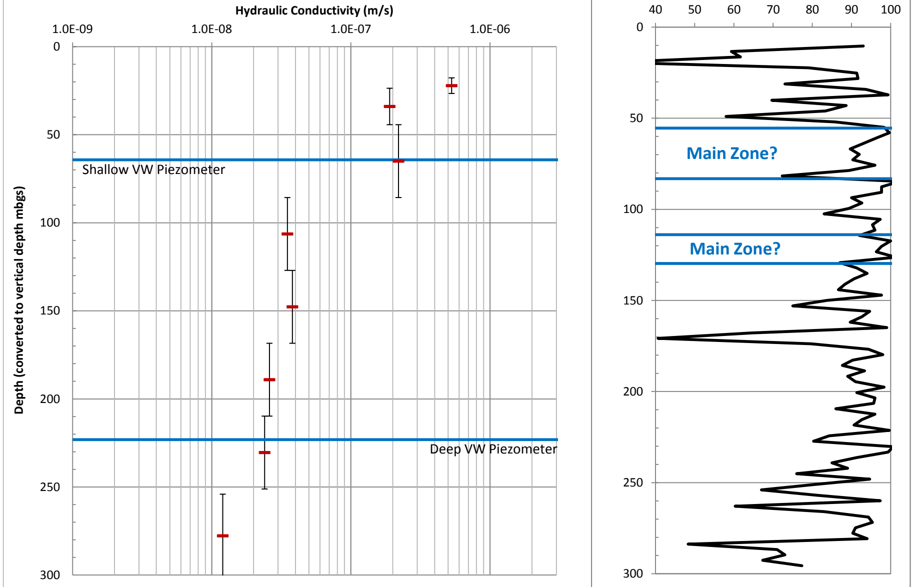
Figure 13a Packer Test Results for Hydrogeology Boreholes from West to East - TL13321
