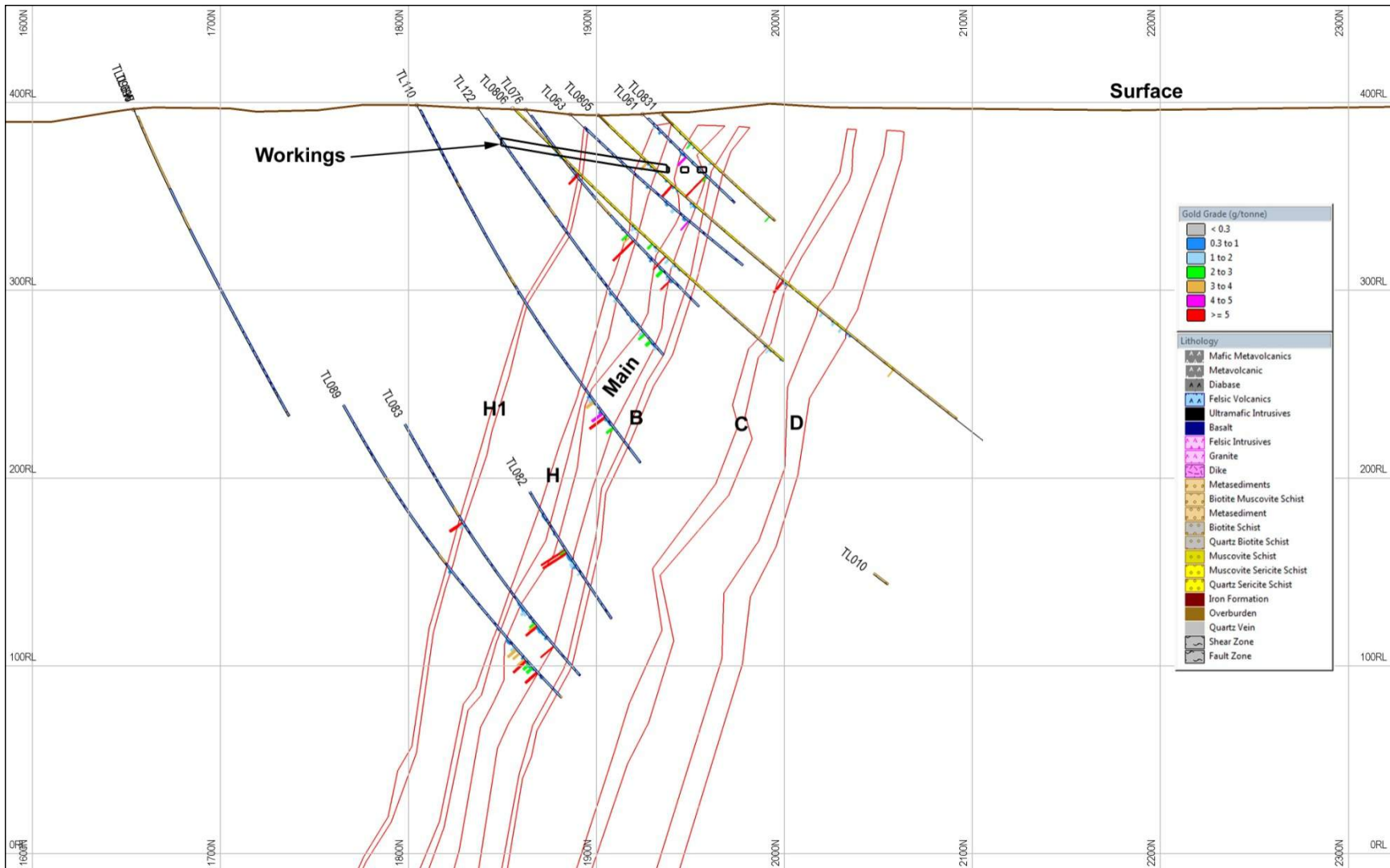
Figure 14-6. Cross-section 7900 m East – facing west.
