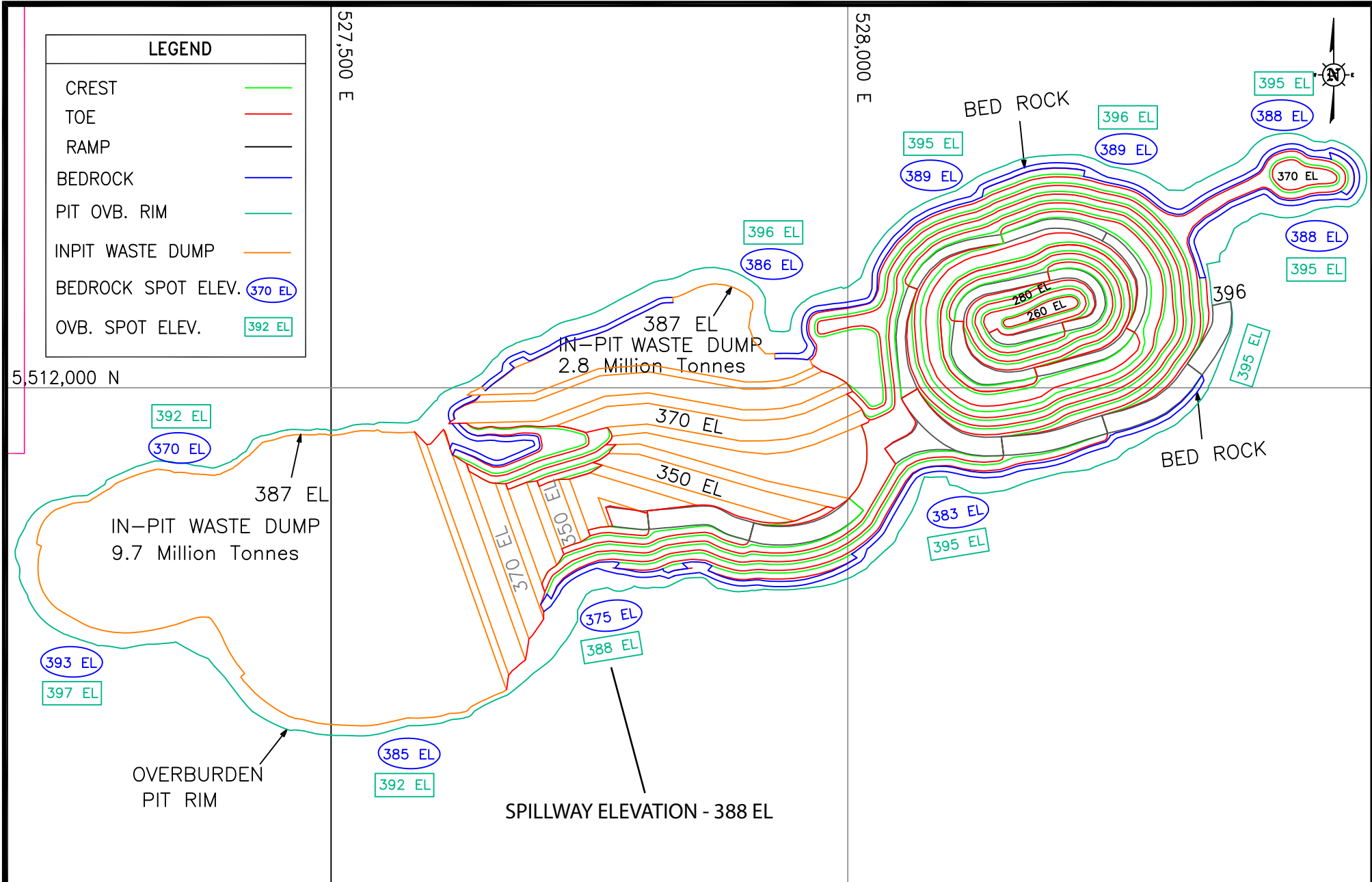
PLAN VIEW GOLIATH ULTIMATE PIT WITH INPIT WASTE ROCK DUMPS
