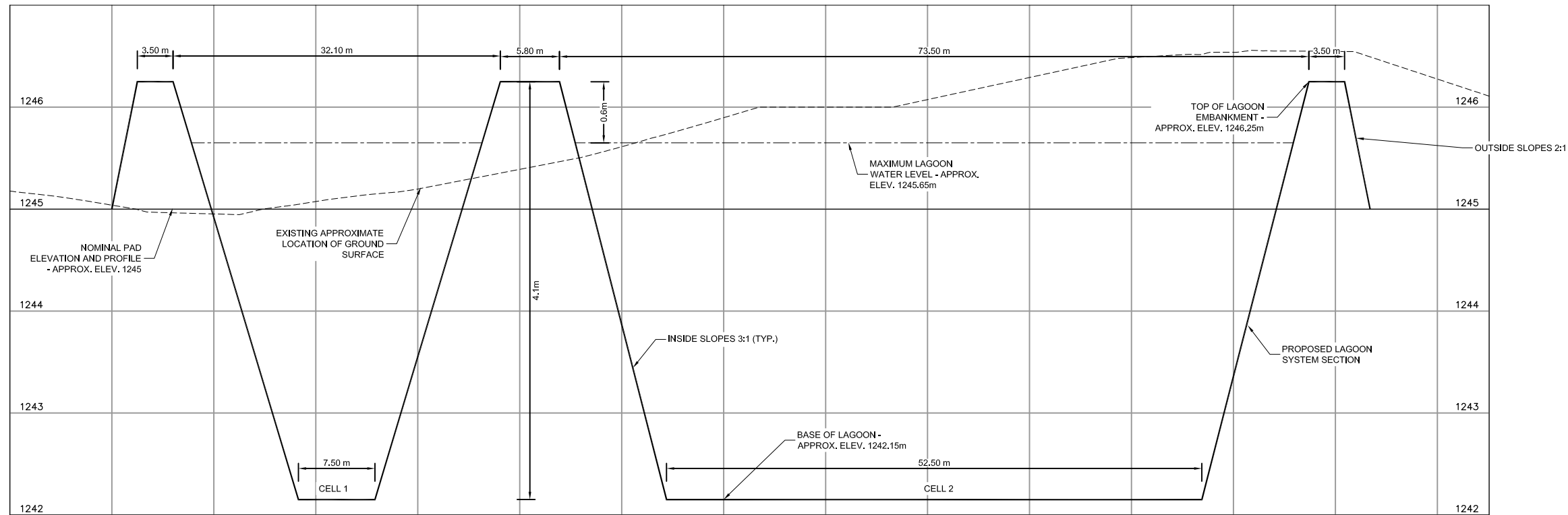
SECTION A 1:500 03
