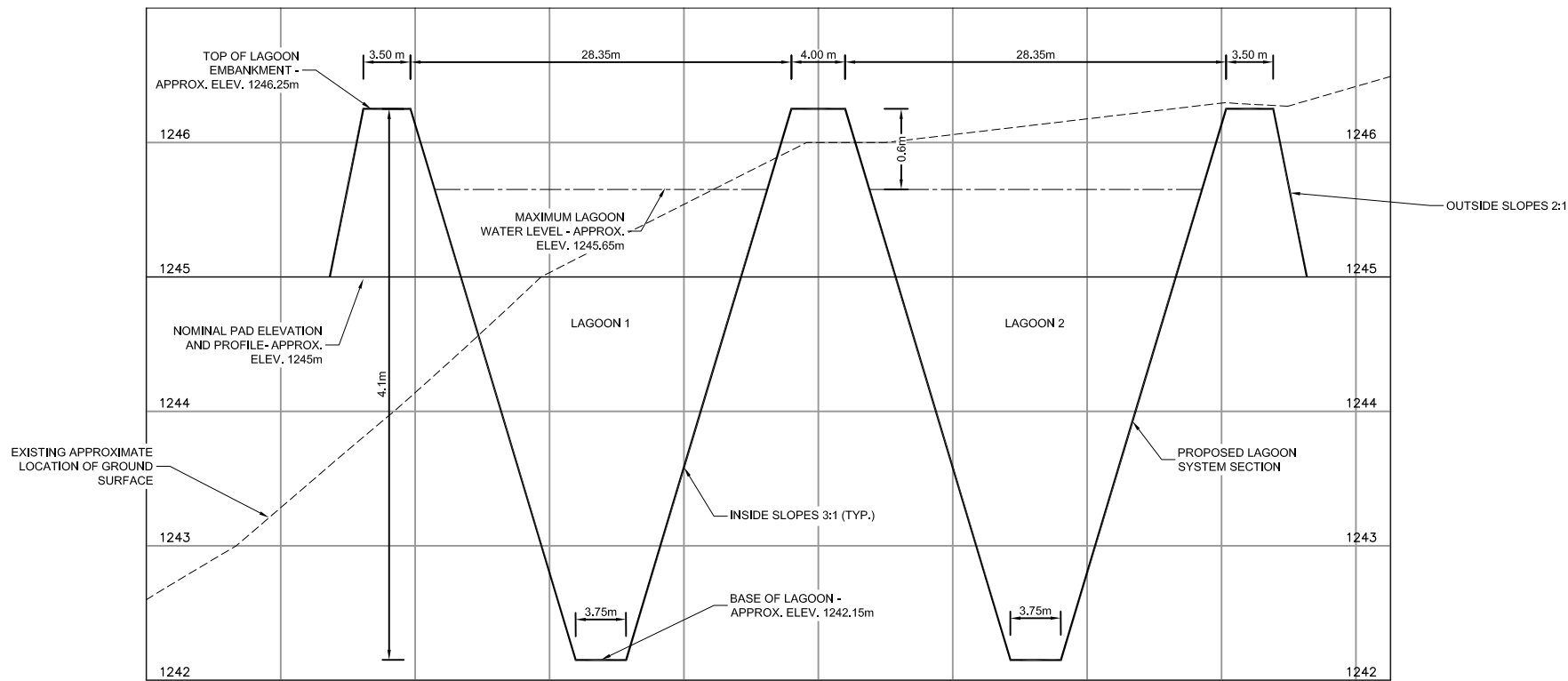
SECTION B 1:500 03
