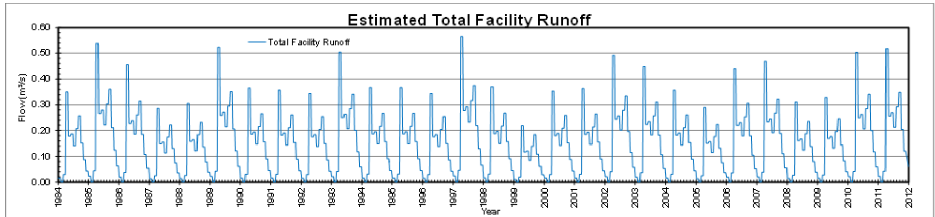
Figure 6-1: Estimated Facility Runoff Flow for Post-closure
