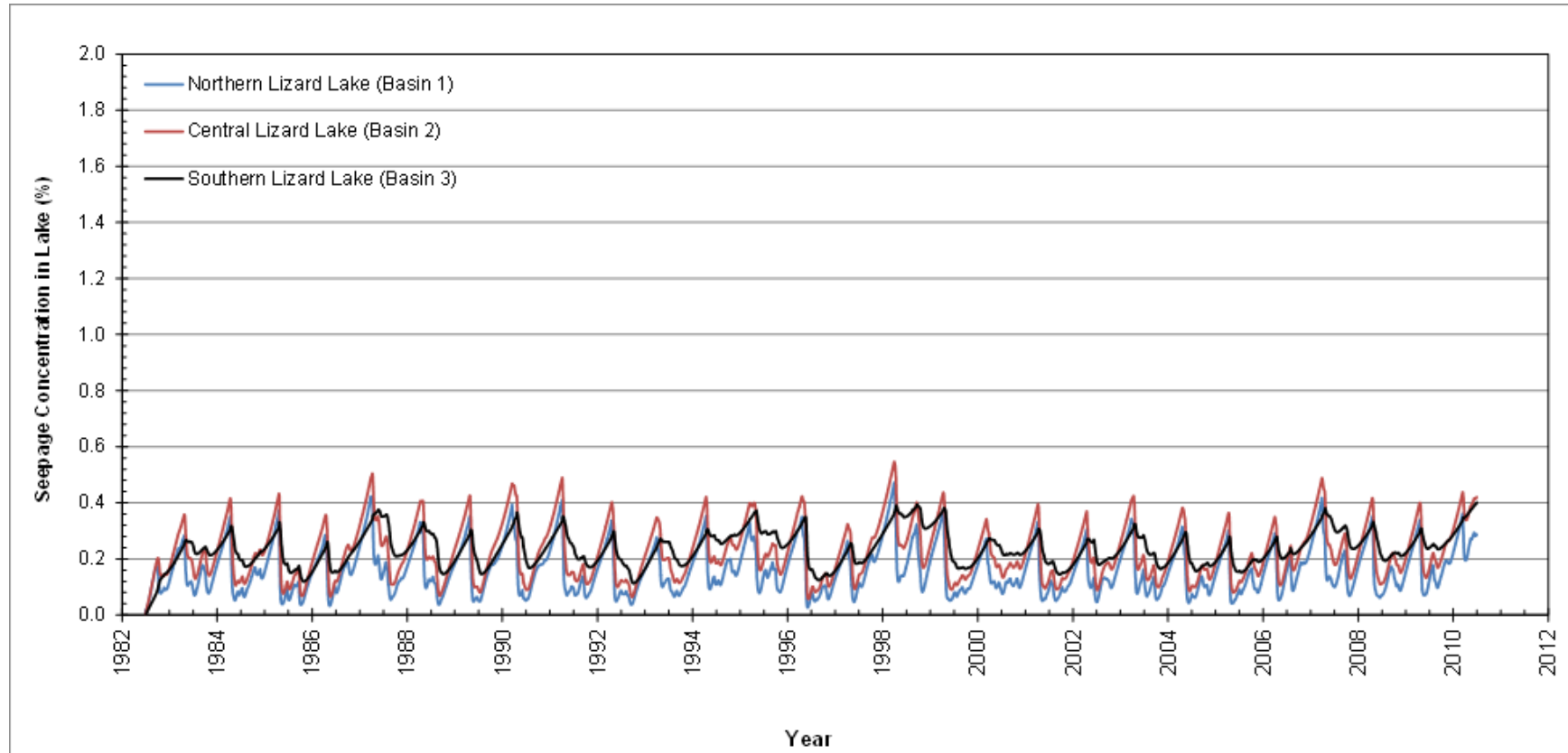
Figure 8-1: Predicted Seepage Concentrations in Lizard Lake for Post-closure
