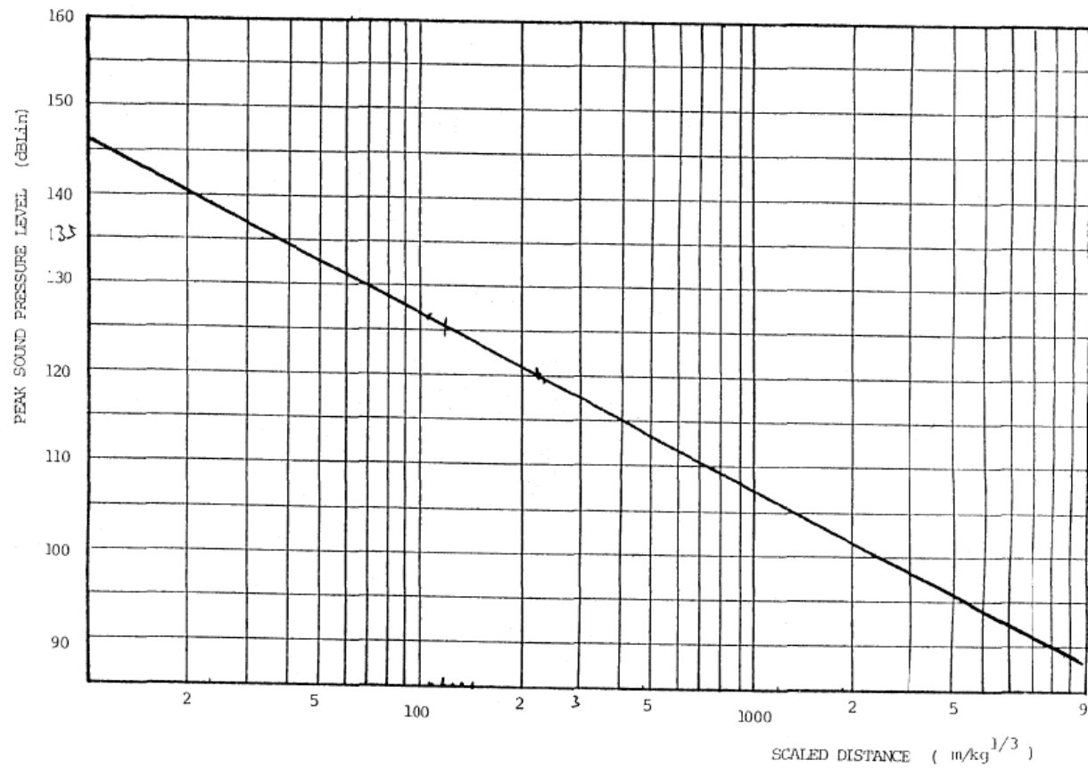
FIGURE 1. BLASTING NOISE PREDICTION
