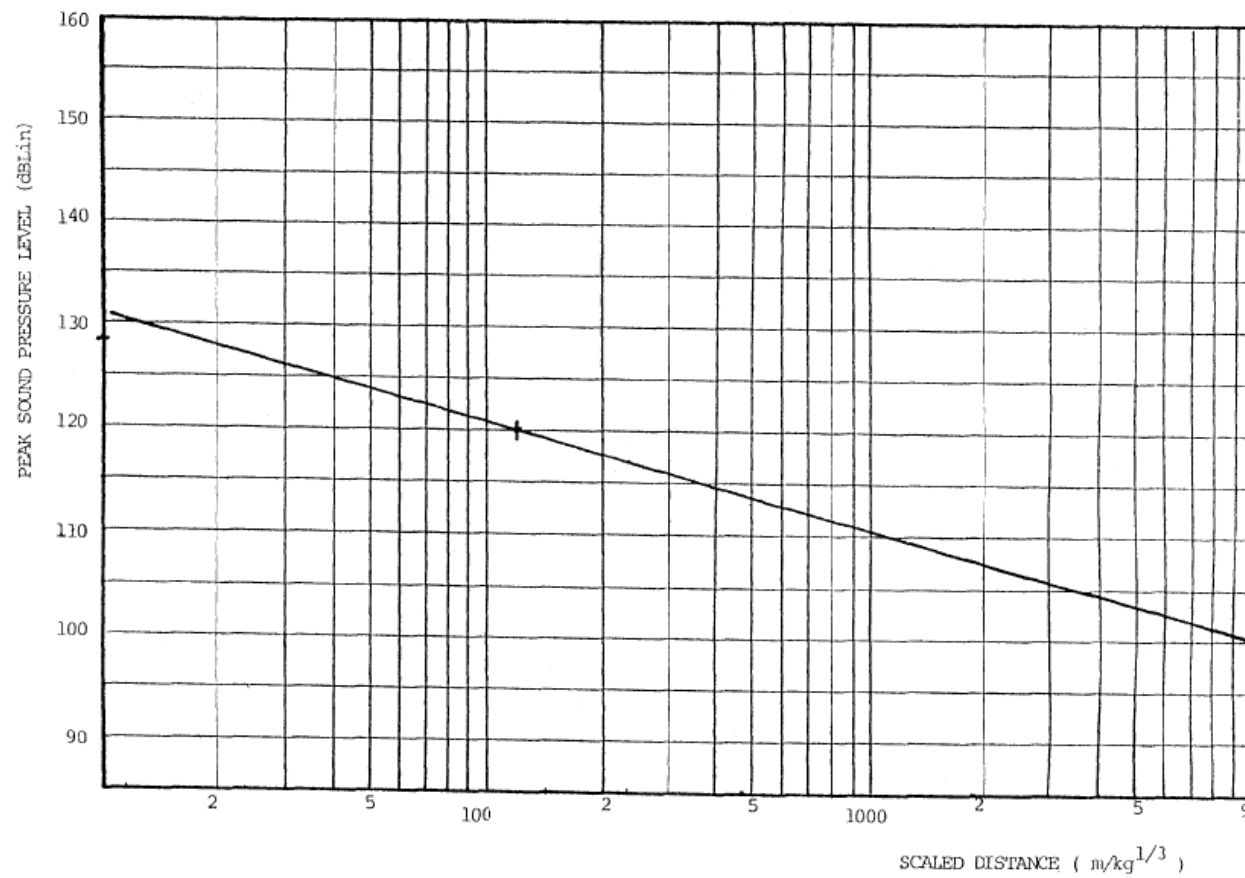
FIGURE 2. BLASTING NOISE PREDICTION
